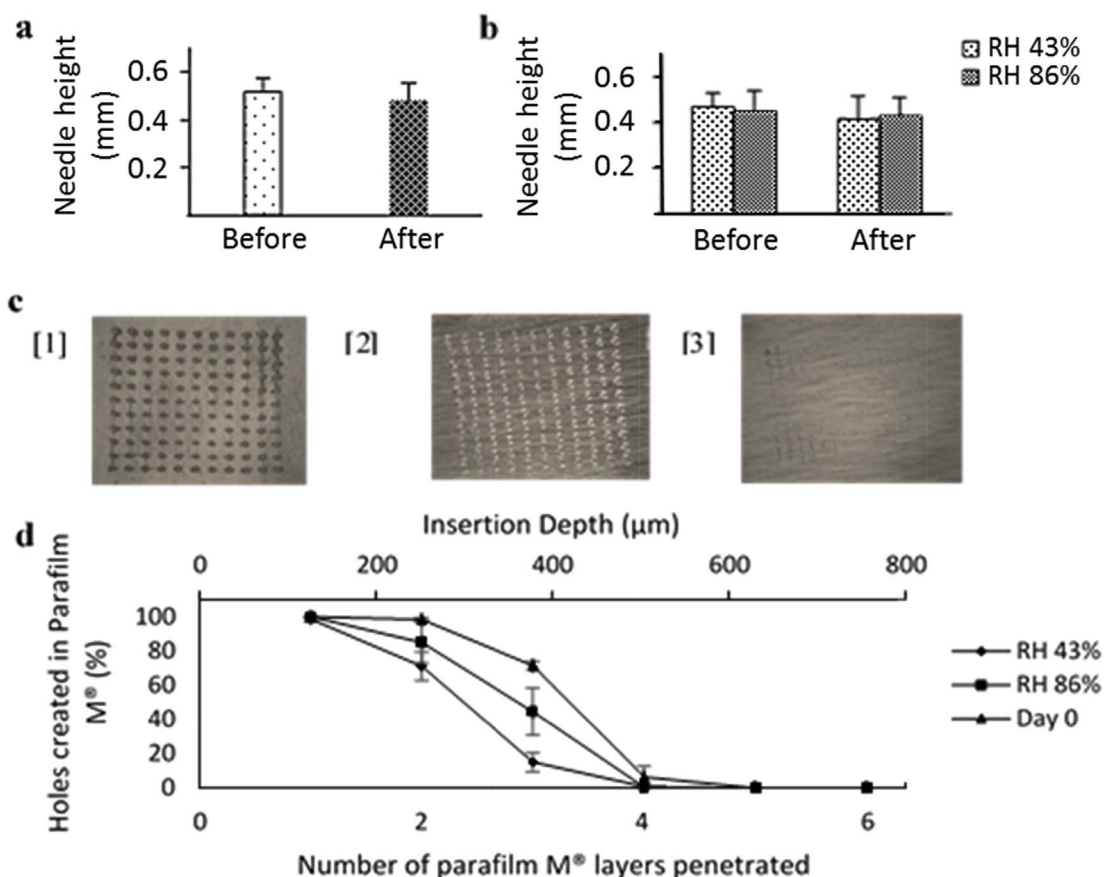
Fig. 2. a) Compression analysis of vitamin K MN arrays, formulated from 20% w/w Gantrez® S-97 and 5% w/w Tween® 80, at day 0. Before compression, needle height was 0.517 ± 0.057 mm (means ± SD, n = 3). After a 32 N force was applied, needle height was 0.480 ± 0.072 mm. b) Comparison of vitamin K MN arrays subjected to RH 43% or RH 86% for 3 days. At RH 43%, before and after compression, needle height was 0.468 ± 0.065 mm and 0.415 ± 0.103 mm respectively (means ± SD, n = 3). RH 86% resulted in needle heights of 0.449 ± 0.093 mm and 0.427 ± 0.086 mm, before and after compression (means ± SD, n = 3). c) Images of the first 3 layers of Parafilm M® used to measure insertion of a vitamin K MN array at day 0. Layers 1 and 2 show 100% needle penetration, with 72% needle penetration through the third layer. d) Number of Parafilm M® layers penetrated and percentage holes created in each layer to enable calculation of mean insertion depth for 3 MN conditions.
