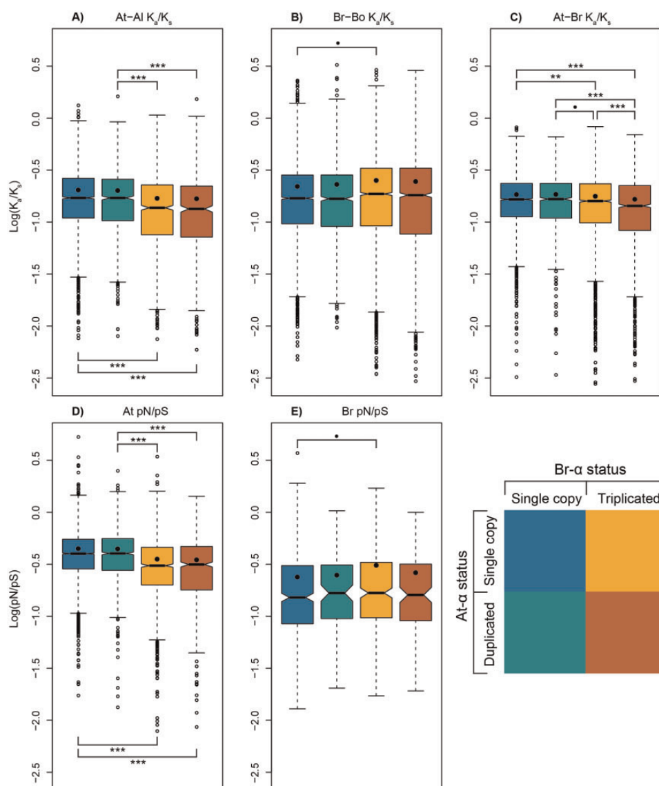
FIG. 2. —Notched box plots of log selective constraints among At-Al-Br-Bo syntenic orthologs. Colors indicate the loss/retention state of Arabidopsis orthologs after At- \alpha WGD, and Brassica orthologs after Br- \alpha WGT. “Lost”: genes returned to singleton state after polyploidy, “retained”: duplicated/triplicated copies are preserved in the genome. Subplots are boxplots of (A) \log(K_a/K_s) for A. thaliana versus A. lyrata , (B) \log(K_a/K_s) for B. rapa versus B. oleracea , (C) \log(K_a/K_s) for A. thaliana versus B. rapa ; and (D) \log(pN/pS) for 1,135 A. thaliana ecotypes, (E) \log(pN/pS) for 126 B. rapa accessions. The notches are 95% confidence intervals of the medians. Kruskal–Wallis multiple comparison tests were performed to evaluate significant differences across medians, P values: *** P < 0.0001 , ** P < 0.001 , * P < 0.01 , • P < 0.05 . The black dots represent the \log(\text{mean}) selective constraints. See also supplementary table S1, Supplementary Material online.
