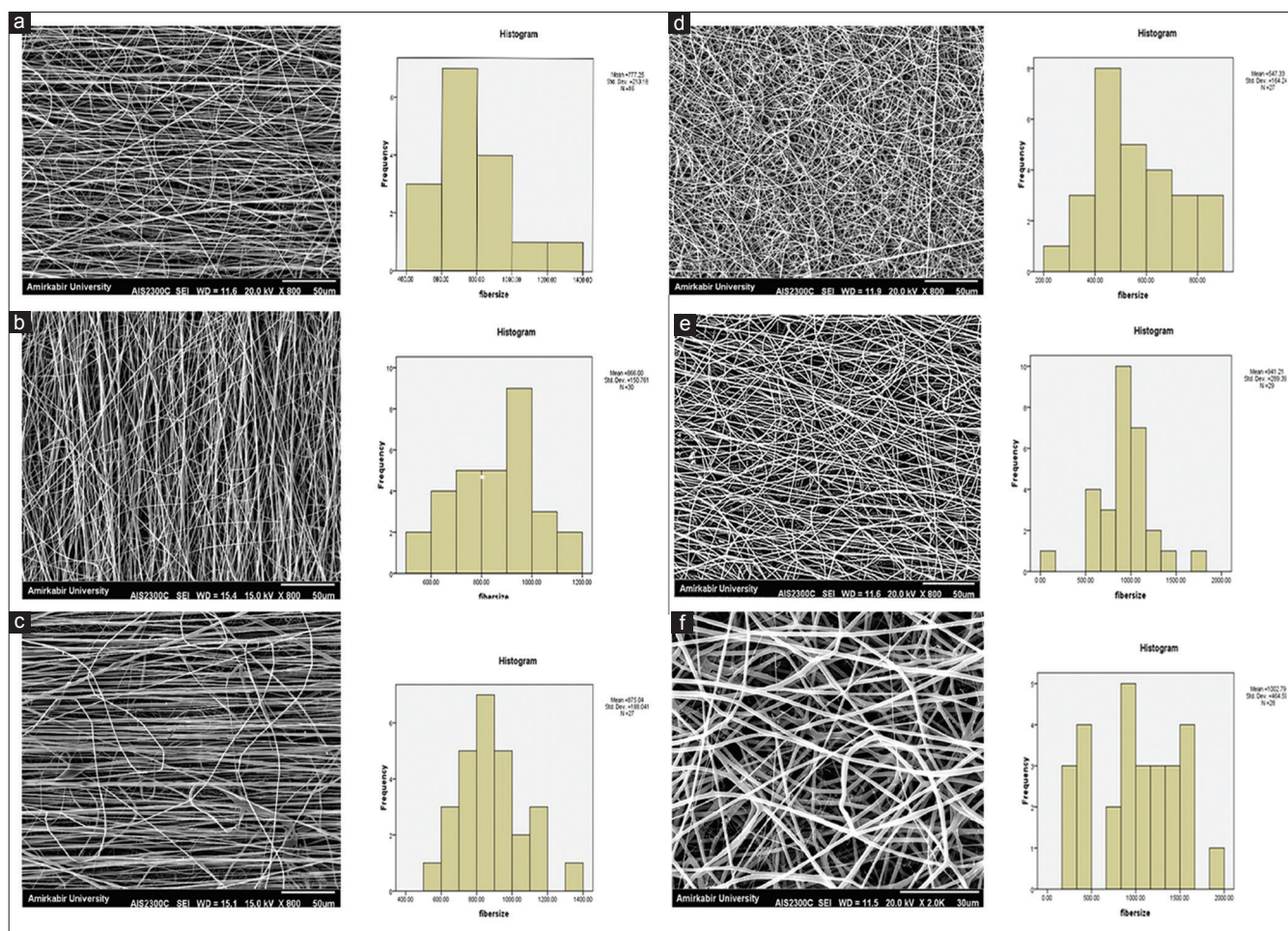
Figure 1: Scanning electron microscopy images of aligned and random pure poly(3-hydroxybutyrate) and poly(3-hydroxybutyrate)/chitosan fibrous scaffolds: (a) Aligned poly(3-hydroxybutyrate), (b) aligned poly(3-hydroxybutyrate)/15% chitosan, (c) aligned poly(3-hydroxybutyrate)/20% chitosan, (d) random poly(3-hydroxybutyrate), (e) random poly(3-hydroxybutyrate)/15% chitosan, (f) random poly(3-hydroxybutyrate)/20% chitosan
