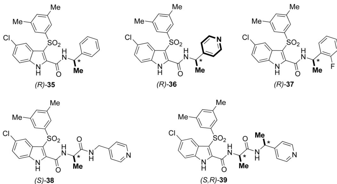
Chart 7. Chiral IASs [35]–[39].
