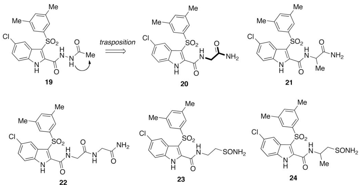
Chart 4. IAS acetylhydrazone [ 19 ] and IASs containing peptide units [ 20 ]–[ 24 ].
