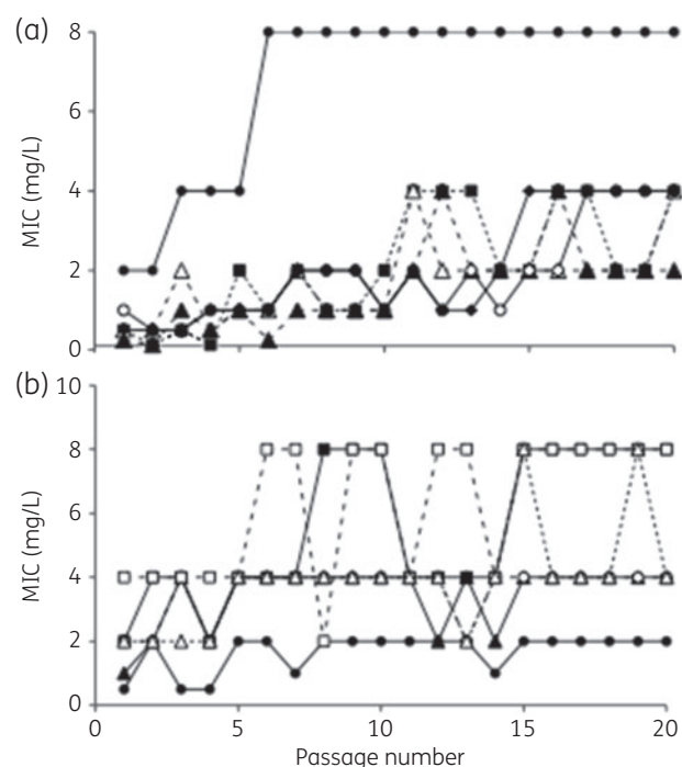
Figure 6. Variation in NAI-107 MICs after serial passages of cultures growing at 0.5 \times MIC. (a) S. aureus strains: squares and broken line, MSSA strain L819; triangles and broken line, MRSA strains L1400 (open symbols) and L4064 (filled symbols); and continuous line, GISA strains L3797 (filled circles), L3798 (open circles) and L4062 (filled diamonds). (b) Enterococcus spp. VanA: filled symbols and broken line, E. faecalis strains A533 (circles), J1 (squares) and A8 (triangles); and open symbols and continuous line, E. faecium strains A6349 (circles), B518 (squares) and D561 (triangles).
