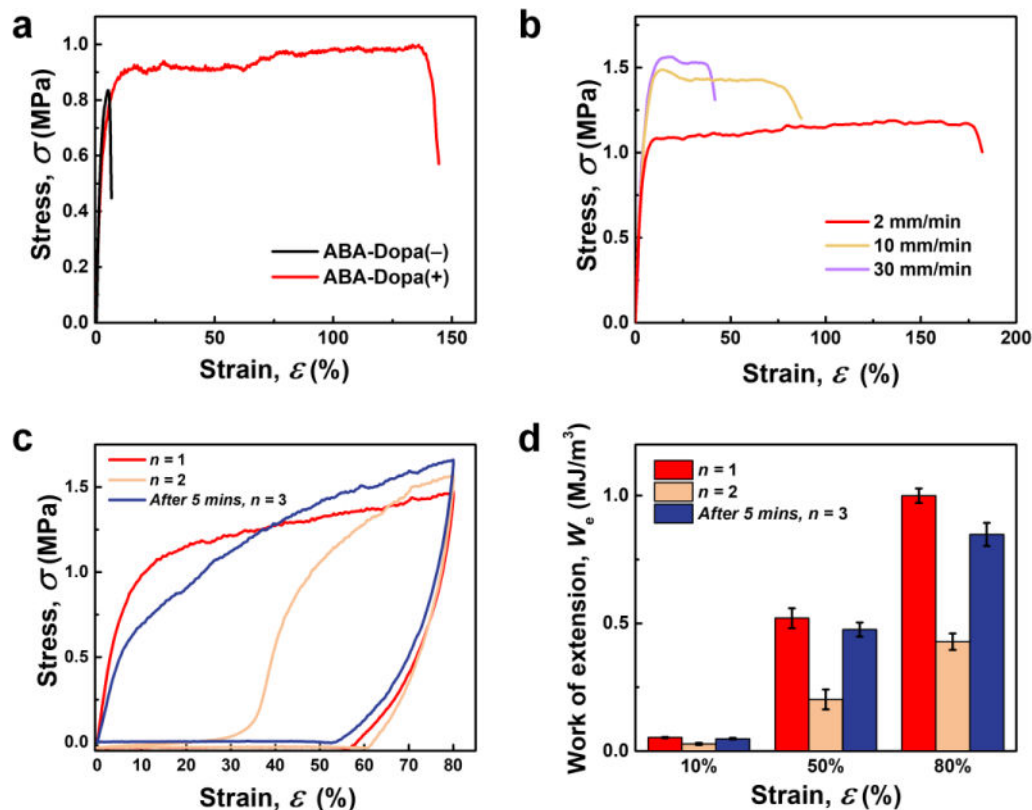
Figure 3. Mechanical properties of networks
