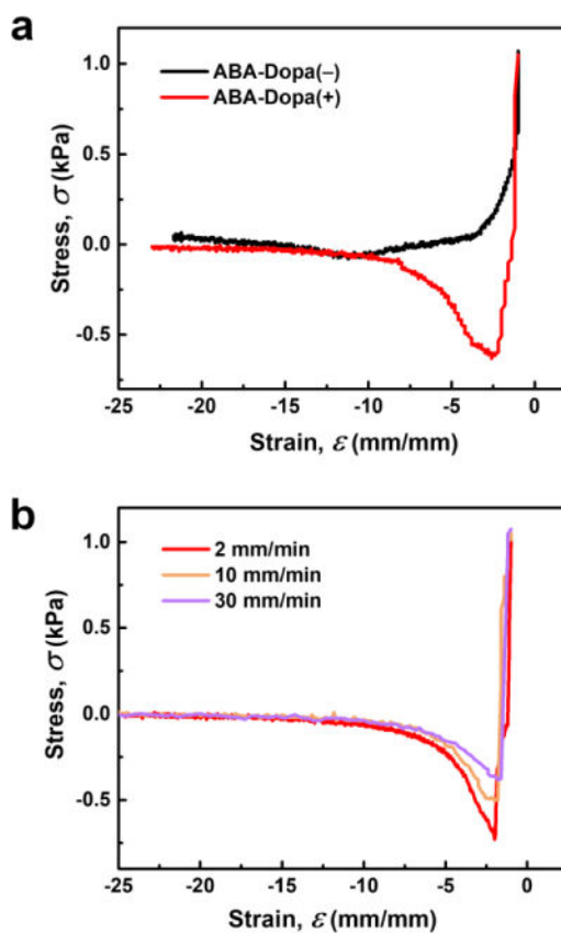
Figure 4. Wet adhesion properties of ABA triblock copolymer networks
