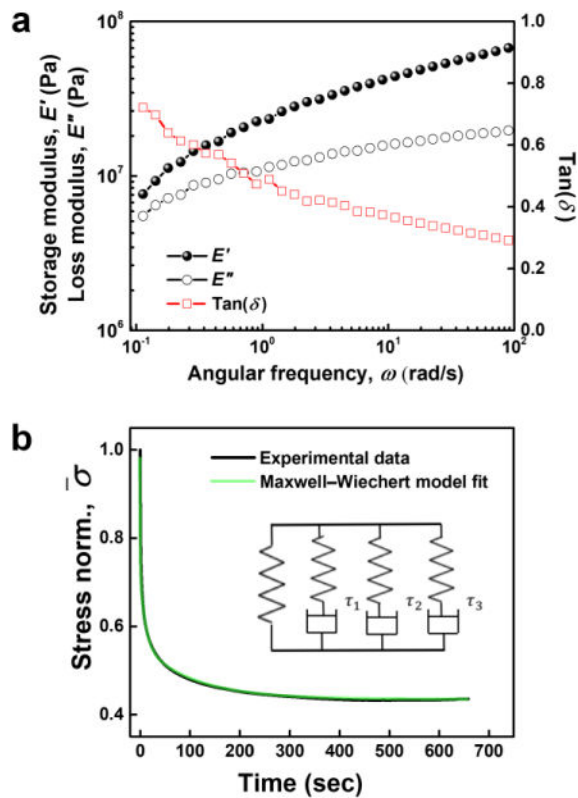
Figure 2. Viscoelastic properties of ABA-Dopa(+) networks comparison to linear viscoelastic models
