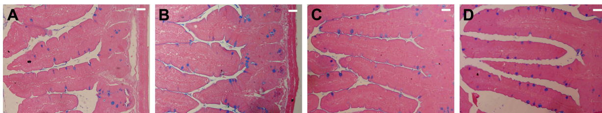
Figure 4 Alcian blue staining of jejunum sections showing goblet cells in (A) control mice, (B) infected mice, and infected mice treated with (C) NaSe and (D) SeNPs. N=5. Scale bar=100 \mu\text{m} .
