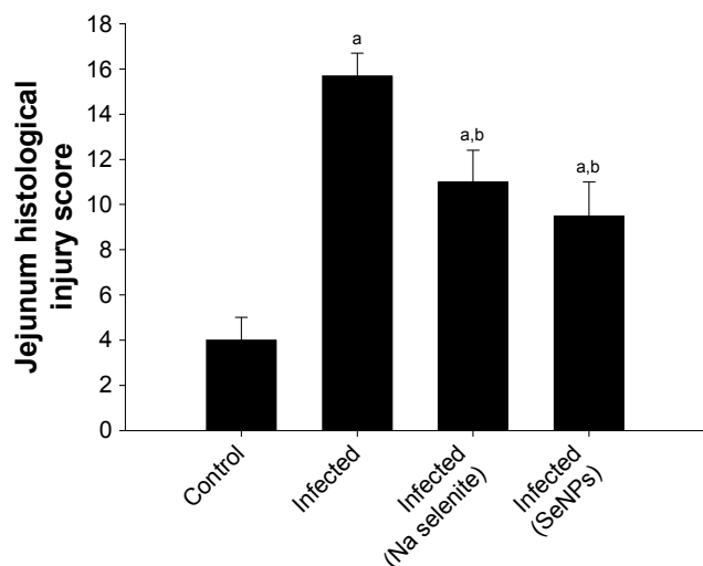
Figure 3 Jejunum histological injury scores on day 5 post-infection for control, non-infected, and infected mice, and for infected mice treated with either NaSe or SeNPs.
