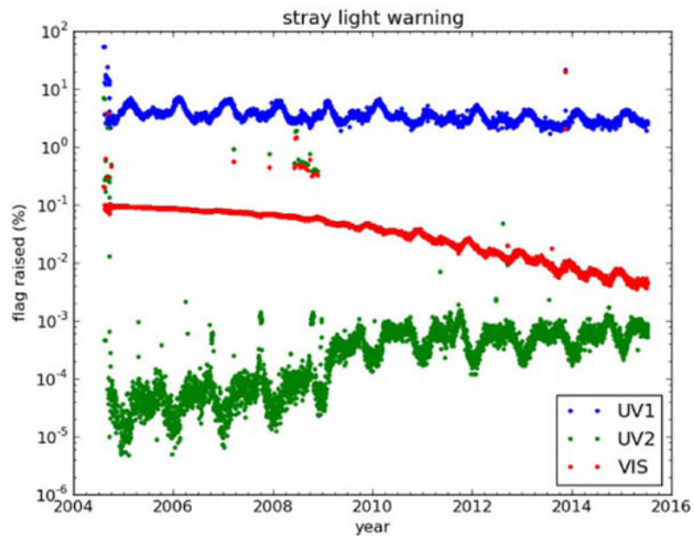
Figure 19. Stray light warning trend over the mission.
