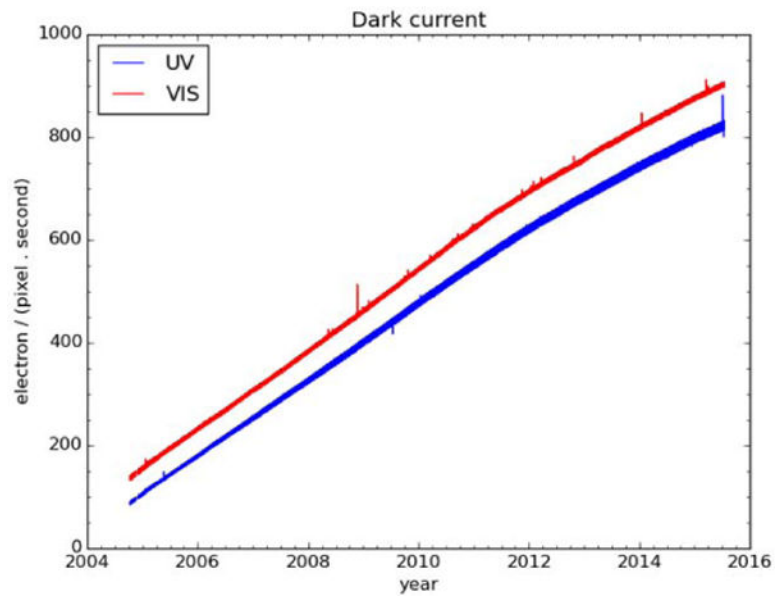
Figure 12. The average dark currents for two CCDs.
