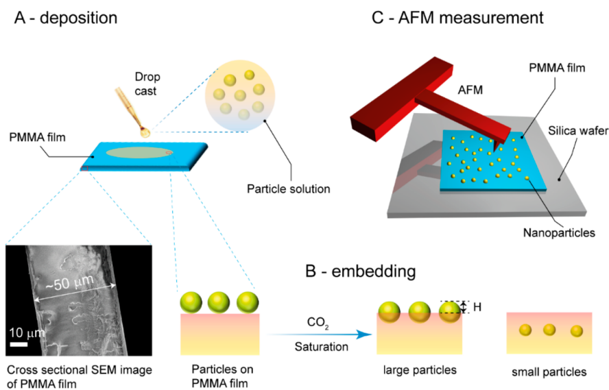
Figure 1. Schematic showing deposition (A) and embedding (B) of nanoparticles on a PMMA film. CO 2 treatment of the particle-laden PMMA layer leads to embedding and even engulfment of the nanoparticles by the polymer layer. The degree by which the particles sink into the PMMA is quantified by measuring the height of nanoparticles above the polymer layer using an AFM (C).
