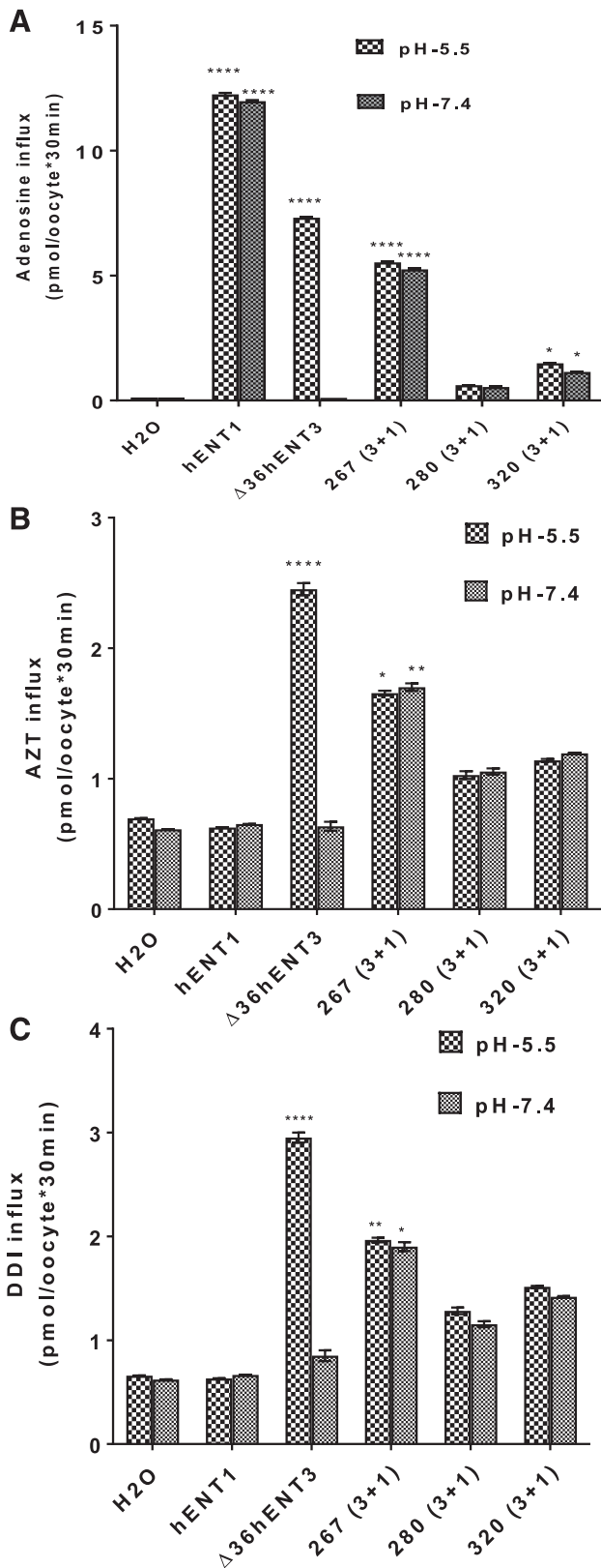
Fig. 3. Identification of the region(s) of hENT3 responsible for 3'-deoxy-nucleoside analog transport by hENT1 and hENT3 chimeras. (A) Uptake of ^3\text{H} -adenosine ( 20\ \mu\text{M} ) into oocytes was measured and plotted at 25^\circ\text{C} 24 hours after injection of hENT1, \Delta 36\text{hENT3} , or chimeric transcripts. (B) Uptake of ^3\text{H} -AZT ( 20\ \mu\text{M} ) into oocytes at 25^\circ\text{C} 24 hours after injection of hENT1, \Delta 36\text{hENT3} , or chimeric transcripts. (C) Uptake of ^3\text{H} -DDI ( 20\ \mu\text{M} ) into oocytes at 25^\circ\text{C} 24 hours after injection of hENT1, \Delta 36\text{hENT3} , and chimeric transcripts. * P < 0.05 ; ** P < 0.01 ; **** P < 0.0001 (one-way analysis of variance). Data represent the average \pm S.E.M. ( n = 8 -12 oocytes).
