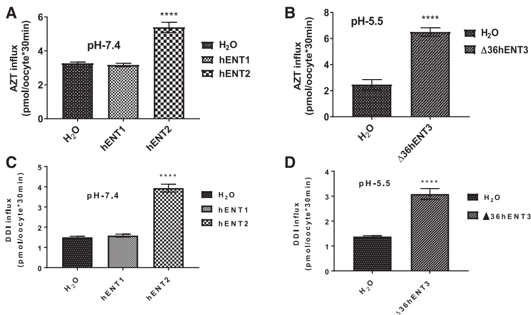
Fig. 1. Determination of the differential 3'-deoxy-nucleoside analog (AZT and DDI) transport by hENTs. (A) Transport activities of 3 H-AZT (20 μM) were measured and plotted at pH 7.4 of oocytes at 25°C 24 hours after injection of H 2 O, hENT1, or hENT2 transcripts. (B) Transport activities of 3 H-AZT (20 μM) at pH 5.5 after injection of oocytes with H 2 O or Δ36hENT3 transcripts. (C) Transport activities of 3 H-DDI (20 μM) were measured and plotted at pH 7.4 of oocytes at 37°C 24 hours after injection of H 2 O, hENT1, or hENT2 transcripts. (D) Transport activities of 3 H-DDI at pH 5.5, with H 2 O or Δ36hENT3 transcript injection. **** P < 0.0001 (one-way analysis of variance/ t test with hENTs compared with H 2 O). Bars represent the average ± S.E. ( n = 8–12 oocytes).
