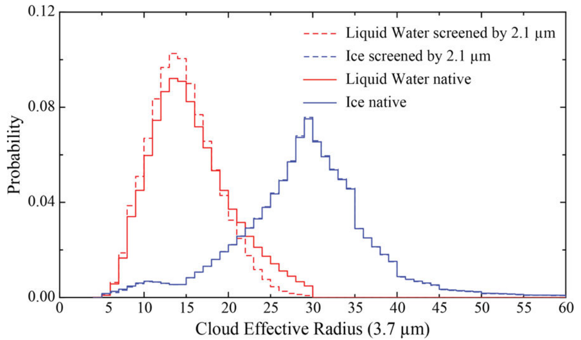
Fig. 9. C6 3.7 μm CER retrieval histograms derived from a Terra MODIS granule obtained on April 1, 2005 (0635 UTC). Here liquid phase (red lines) and ice phase (blue lines) histograms are shown for C5 (dashed lines) and C6 (solid lines). The C5 removal of successful spectral CER retrievals due to filtering by successful 2.1 μm retrievals leads to a systematic shift in the CER retrieval histogram.
