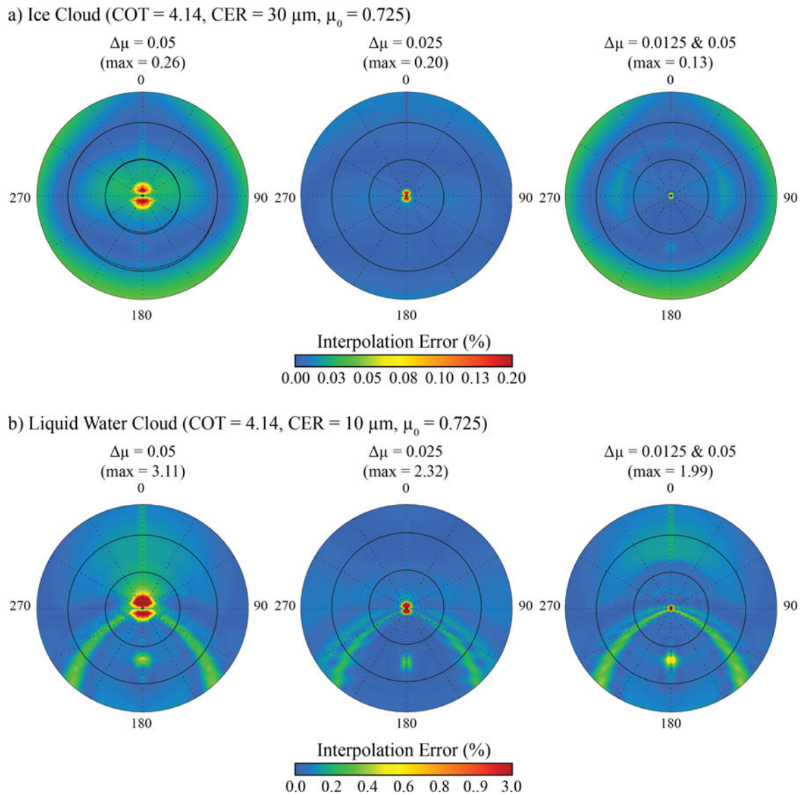
Fig. 2. Maximum multiple scattering reflectance interpolation error for COT = 4.14 and \mu_0 = 0.725 for (a) ice clouds with CER = 30 \mu\text{m} (severely roughened aggregated columns) and (b) liquid water clouds with CER = 10 \mu\text{m} . The hybrid LUT discretization scheme adopted for C6 (right column) has the least error near nadir.
