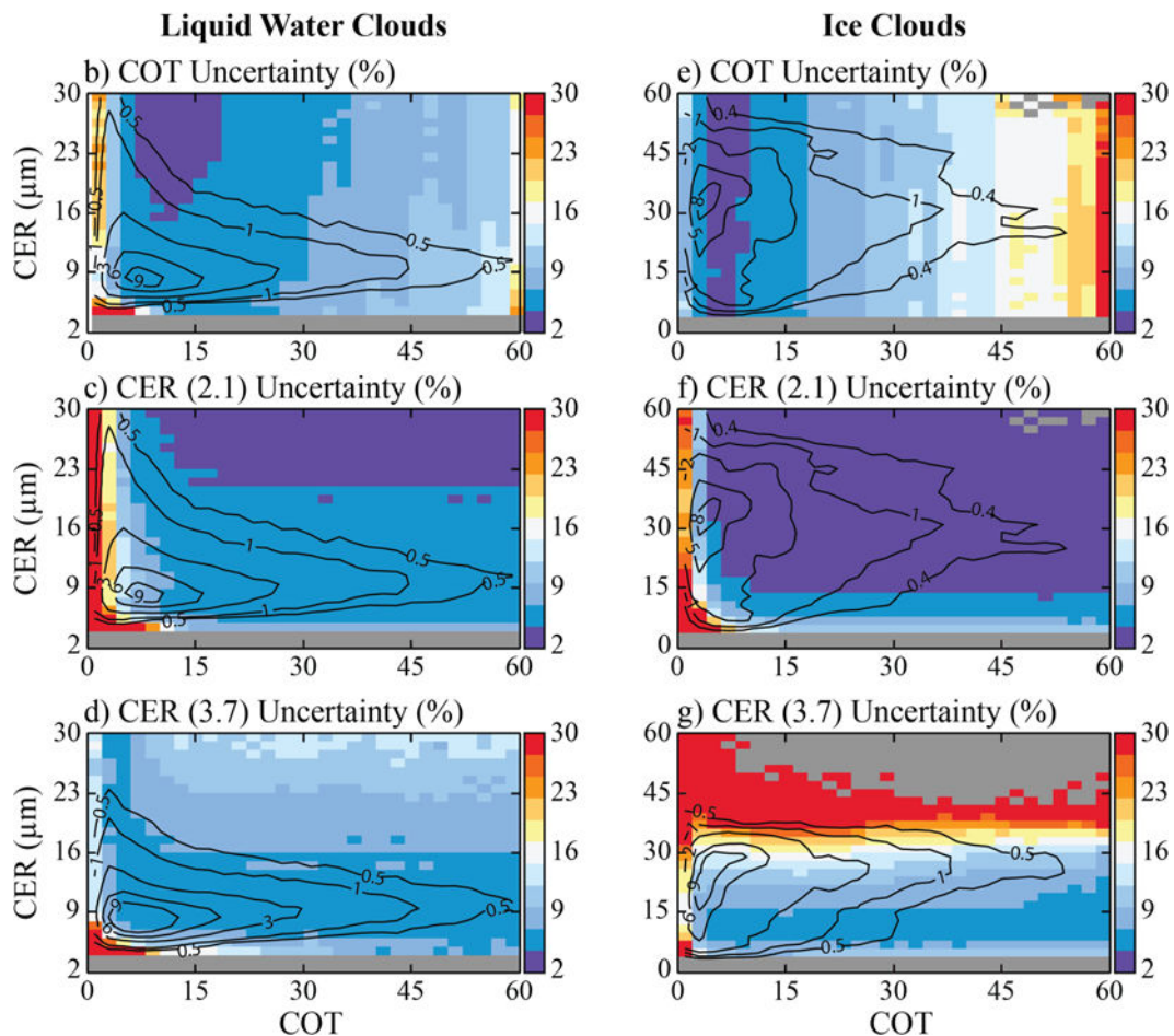
Fig. 13. Total calculated mean liquid water and ice cloud retrieval uncertainties binned as a function of COT and CER for all successful retrievals from the central U.S. granule shown in (a). COT uncertainties (b, e) are relatively higher at small and large COT with sensitivity to CER only for the smallest sizes. CER uncertainties (c,d,f,g) are generally higher at small COT and CER. Grey-shaded bins either indicate effective radius values outside the LUT or the absence of pixels in the granule with that COT-CER retrieval pair. Contours of normalized retrieval counts for the COT and CER pairs are also shown.
