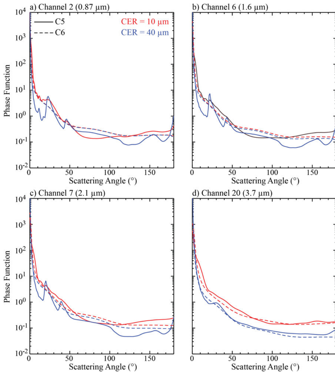
Fig. 6. C5 (solid line) and C6 (dashed line) ice model phase functions at four wavelength channels for CER = 10 \mu\text{m} (red) and 40 \mu\text{m} (blue).
