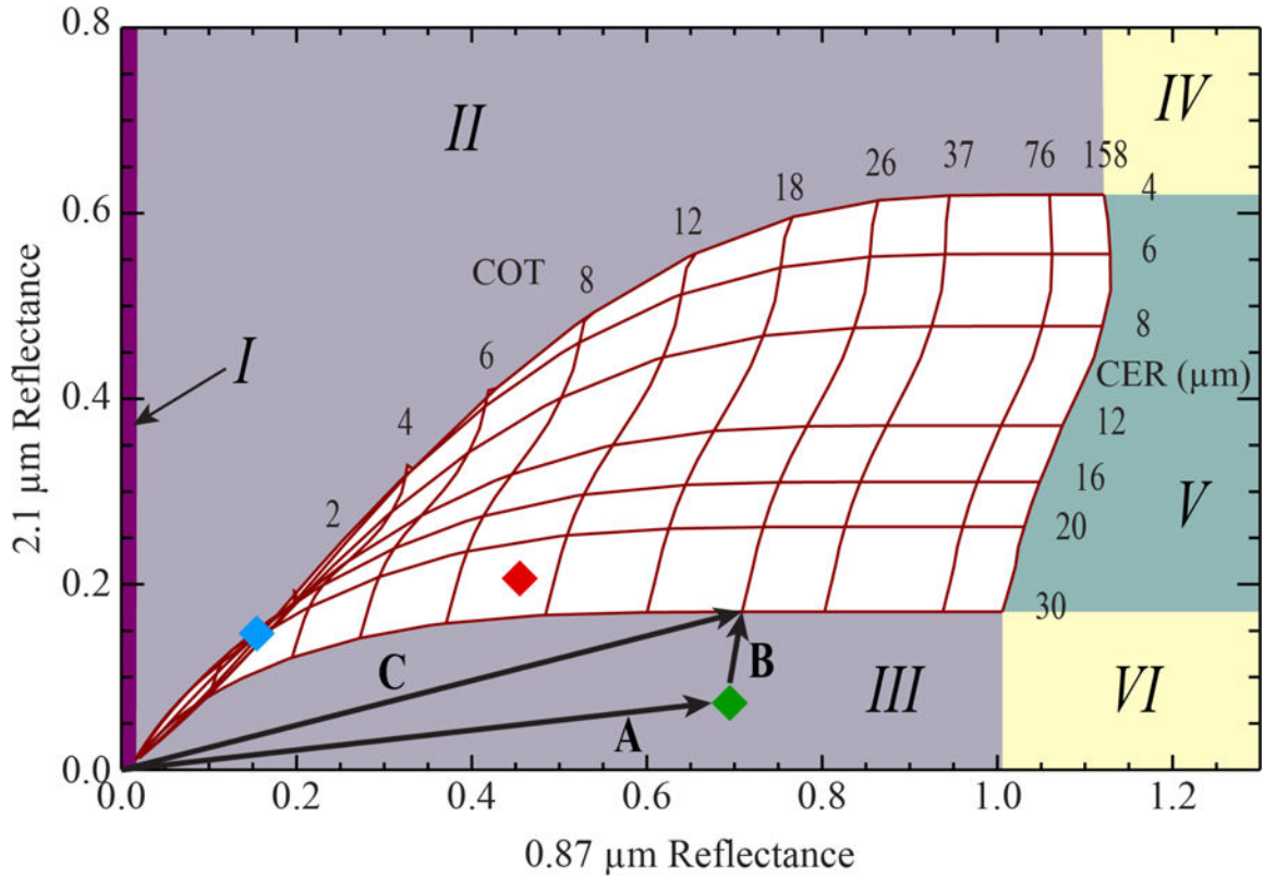
Fig. 11. Retrieval space for a liquid phase cloud over an ocean surface ( \theta_0 = 19.89^\circ , \theta = 22.39^\circ , \Phi = 174.4^\circ , wind speed = 7 \text{ m}\times\text{s}^{-1} ), highlighting Retrieval Failure Metric (RFM) categories and cost metric assignments (see Table III). Also shown are example pixels illustrating a successful retrieval (red marker), a retrieval outside the solution space (green), and a multiple CER solution retrieval (blue). The vectors A , B , and C are used for computing the cost metric (3) for the pixel outside the solution space. The same logic also applies to ice cloud retrievals (see example solution space in Fig. 7).
