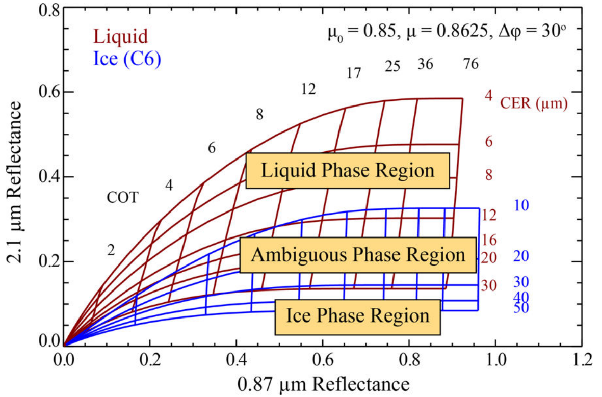
Fig. 7. The theoretical relationship between top-of-cloud reflectance in the 0.87 and 2.1 \mu\text{m} MODIS channels for liquid water (red) and the C6 ice cloud model (blue) for various values of COT and CER. Reflectance observations can occur in regions of the solution space that are unambiguously liquid or ice, but may also lie in regions that are ambiguous regarding phase.
