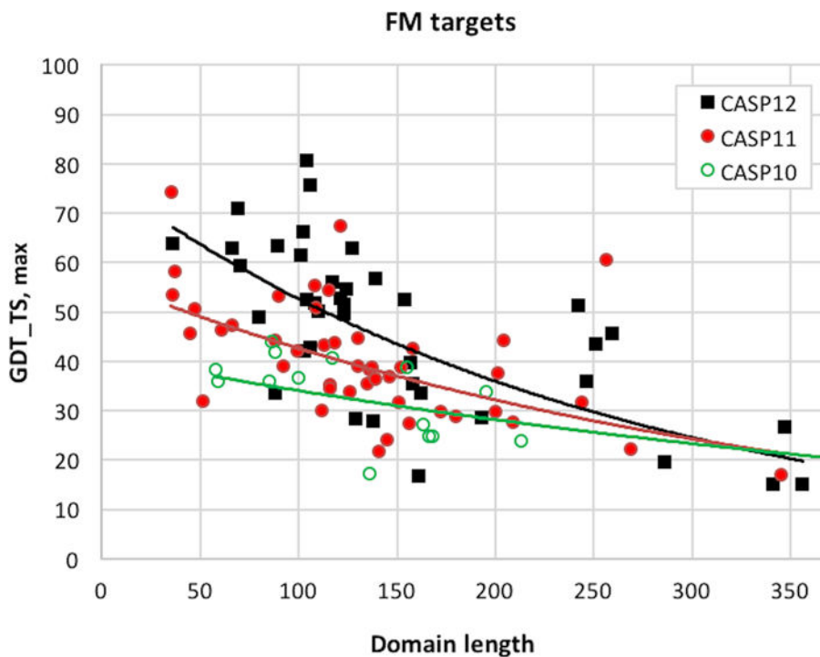
Figure 2. Backbone accuracy (GDT_TS) of the best submitted models in the free modeling category for the three most recent CASPs, as a function of target length. Good performance for targets smaller than 100 residues mostly reflects earlier improvements in this category. In CASP10, no models longer than 100 residues had GDT_TS greater than 50. In CASP11, four crossed this threshold. In CASP12, half of the targets longer than 100 residues do so. (On the GDT_TS scale, 100 is perfect agreement with experiment, 20 – 30 is typically random, and structures with scores above 50 are largely topologically correct).
