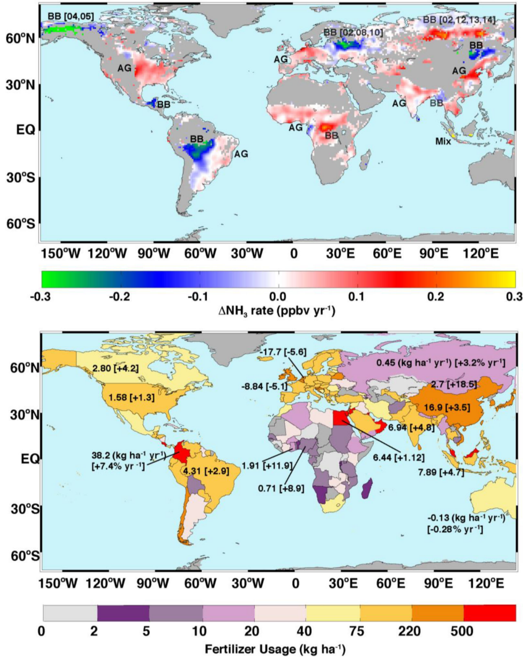
Figure 1. Trend in AIRS NH 3 Top: Temporal trends (+ 0.3 to -0.3 ppbv yr -1 ). The locations and the last two digits of the years of biomass burning events (in square brackets) are marked as BB. The main agricultural regions are marked as AG. Bottom: national averaged annual N fertilizer usage in 2002 – 2013 in kg ha -1 and trends [percentage changes] in kg ha -1 yr -1 [% yr -1 ]; see text for details.
