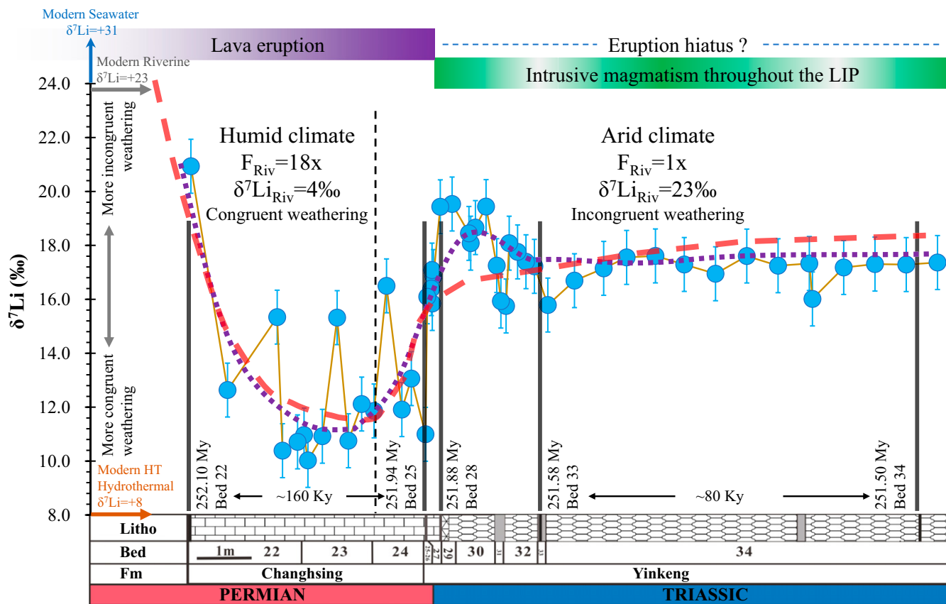
Fig. 2. Seawater \delta^7\text{Li} at the PTB and dynamic modeling fit to the observed data. Model line (red dashed line) represents the variation of lithium isotope composition of seawater corresponding to enhanced weathering pulse (with 18\times Li flux and \delta^7\text{Li} \sim 4\text{‰} ) started before Beds 22–23 for \sim 300 Ky and subsequent decrease in weathering rate (with 1\times Li flux and \delta^7\text{Li} \sim 23\text{‰} ) from Bed 24 to Bed 34 for \sim 400 Ky. Purple dotted line is the smoothed seawater Li isotopic trend. Detailed modeling parameters can be found in SI Appendix, Table S3 . The modeling suggests climate change from humid to arid at PTB, which is consistent with the eruption time of the Siberian Traps. Dashed black line corresponding to the early stage of Bed 24 represents the change of modeling parameters. Timeline of Siberian Traps LIP magmatism (purple and green bands) and dated ash beds from the Meishan section (black bars) are from refs. 25 and 46.
