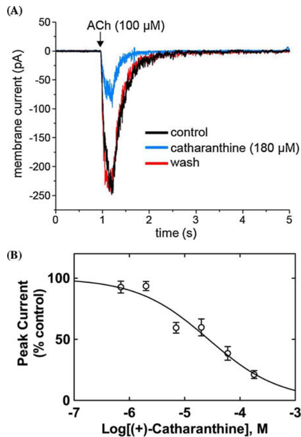
Fig. 5. Inhibitory potency of (+)-catharanthine on ACh-evoked currents from MHb (VI) neurons. (A) ACh puffer (100 \mu\text{M} )-evoked currents from MHb (VI) neurons are decreased by 180 \mu\text{M} (+)-catharanthine. The puffer was performed for 250 ms at a pressure of 12 psi. After washing (10 min), the peak amplitude reached the same levels as that observed in control neurons, indicating a reversible inhibition. (B) Concentration-response relationship for the inhibitory activity of (+)-catharanthine on MHb (VI) neurons. Response was normalized to the maximal ACh response which was set as 100%. The plot ( r^2 = 0.87 ) is representative of 4–7 determinations, where the error bars are the S.D. The calculated \text{IC}_{50} and n_{\text{H}} values are summarized in Table 2.
