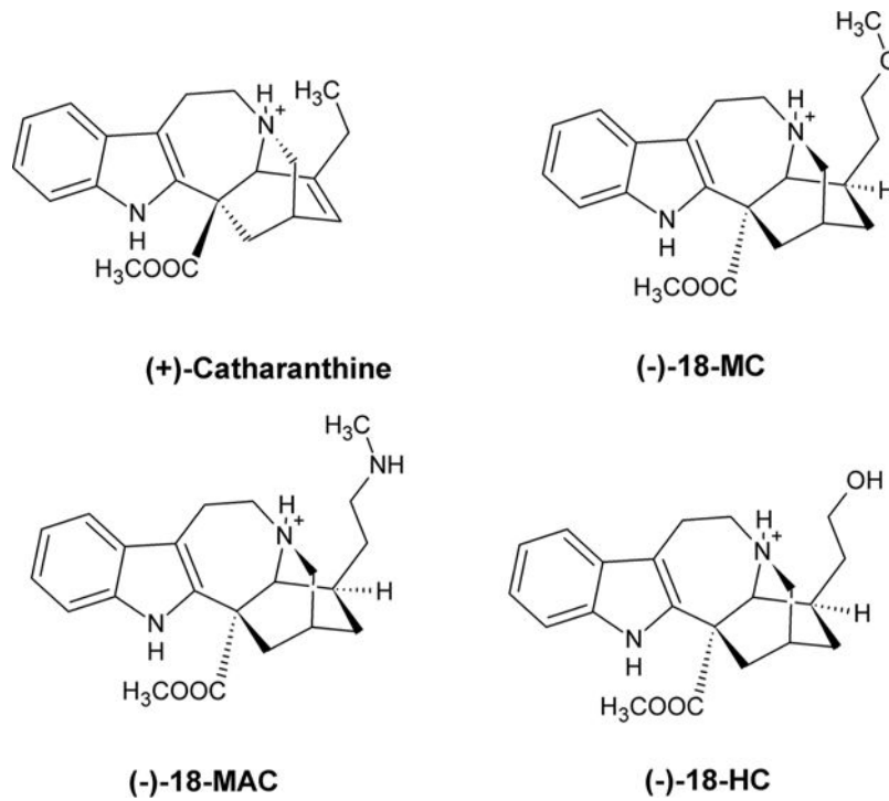
Fig. 1. Molecular structure of coronaridine congeners in the protonated state, including (-)-18-MC [(-)-18-methoxycoronaridine], (-)-18-HC [(-)-18-hydroxycoronaridine], (-)-18-MAC [(-)-18-methylaminocoronaridine], and (+)-catharanthine [(+)-3,4-didehydrocoronaridine].
