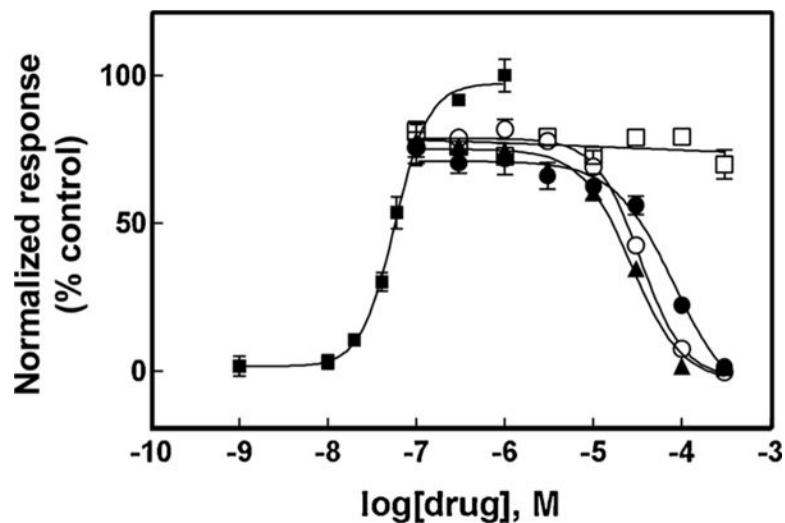
Fig. 3. Effect of coronaridine congeners on (±)-epibatidine-induced \text{Ca}^{2+} influx in GH3- \alpha 7 cells. Increased concentrations of (±)-epibatidine (■) activated \alpha 7 AChRs with potency \text{EC}_{50} = 26 \pm 4 nM ( n = 25 ). Subsequently, cells were pre-treated (5 min) with several concentrations of (+)-catharanthine (▲), (±)-18-MC (○), (±)-18-MAC (□), and (±)-18-HC (●), followed by addition of 1.0 \mu\text{M} (±)-epibatidine. Response was normalized to the maximal (±)-epibatidine response which was set as 100%. The plots are representative of four determinations, where the error bars are the S.D. The calculated \text{IC}_{50} and n_{\text{H}} values are summarized in Table 1.
