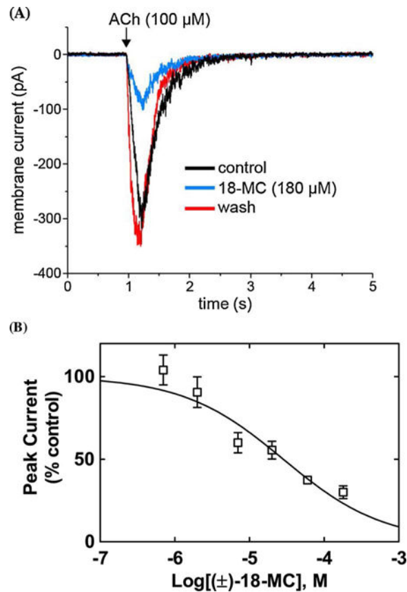
Fig. 4. Inhibitory potency of (±)-18-MC on ACh-evoked currents from MHb (VI) neurons. (A) ACh puffer (100 μM)-evoked currents from MHb (VI) neurons are decreased by 180 μM (±)-18-MC. The puffer was performed for 250 ms at a pressure of 12 psi. After washing (13 min), the peak amplitude reached the same levels as that observed in control neurons, indicating a reversible inhibition. (B) Concentration-response relationship for the inhibitory activity of (±)-18-MC on ACh-evoked currents from MHb (VI) neurons. Response was normalized to the maximal ACh response which was set as 100%. The plot ( r^2 = 0.80 ) is representative of 5–7 determinations, where the error bars are the S.D. The calculated IC_{50} and n_H values are summarized in Table 2.
