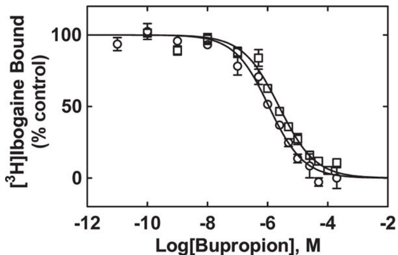
Fig. 6. Bupropion-induced inhibition of [ ^3\text{H} ]ibogaine binding to \text{h}\alpha 3\beta 4 AChRs in the resting ( \square ) and desensitized ( \circ ) states, respectively. \text{h}\alpha 3\beta 4 AChR membranes (1.5 mg/mL) were pre-incubated (30 min) with 16.6 nM [ ^3\text{H} ]ibogaine in the absence (receptors are mainly in the resting state) and presence of 1 \mu\text{M} (–)-nicotine (receptors are mainly in the desensitized state), and then equilibrated with increasing concentrations of bupropion. Nonspecific binding was determined at 100 \mu\text{M} (–)-ibogaine. The plots are combinations of two experiments, each performed in triplicate, where the error bars are the S.D. The \text{IC}_{50} and n_{\text{H}} values were obtained by nonlinear least-squares fit of the plots ( r^2 = 0.95 for both). The K_{\text{i}} values, calculated using eq. 1 and summarized in Table 3, indicated that bupropion binds to desensitized \text{h}\alpha 3\beta 4 AChRs with higher affinity than that at resting receptors (Student t -test p = 0.001 ).
