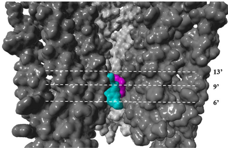
Fig. 7. Model of the h \alpha 3 \beta 4 AChR transmembrane domain showing the ion channel lumen (modified from Arias et al., 2010b). (-)-Ibogaine (cyan) interacts with a luminal site formed between the phenylalanine/valine (position 13') and serine (position 6') rings (Arias et al., 2010b), which overlaps the site for (-)-bupropion (magenta) (Arias et al., submitted manuscript). The AChR and ligands are depicted by its solvent accessible surface.
