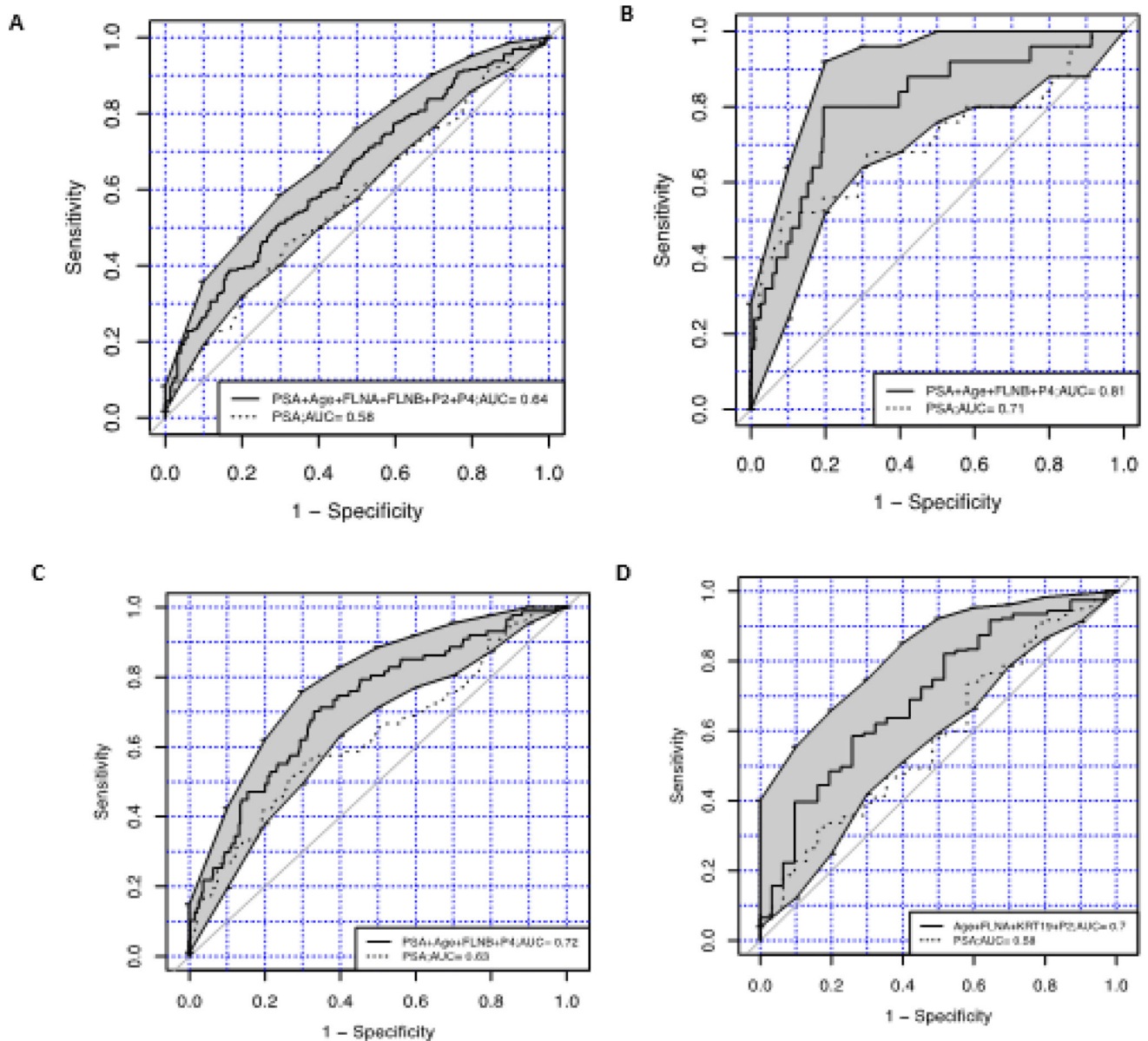
Figure 1. ROC curves of regression models using the prostate biomarker panel, age and PSA test compared to PSA alone
