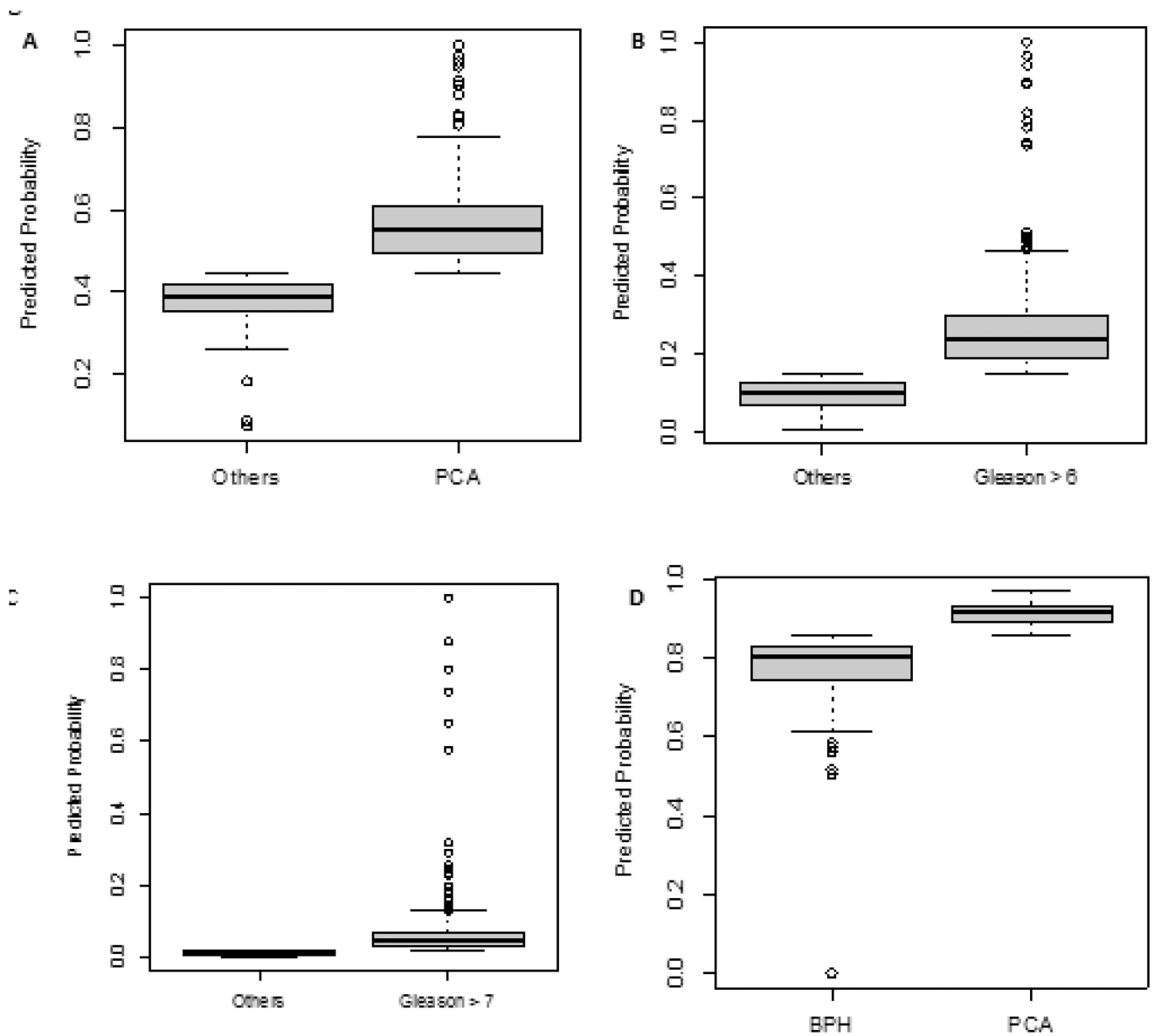
Figure 2. Predicted probability distributions plotted for each ROC analysis
