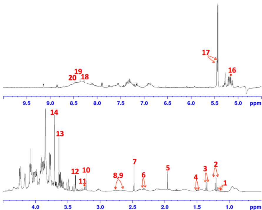
Figure 2: Representative 1 H-NMR Spectrum of the total region of aquafaba. 1, Isopropanol; 2, ethanol; 3, lactic acid; 4, alanine; 5, acetic acid; 6, glutamine; 7, succinic acid; 8, citrate; 9, malate; 10, choline; 11, phosphocholine; 12, methanol; 13, sucrose; 14, glucose; 15, β-glucose; 16, α-glucose; 17, sucrose; 18, inosine; 19, adenosine; 20, formate. Please click here to view a larger version of this figure.
