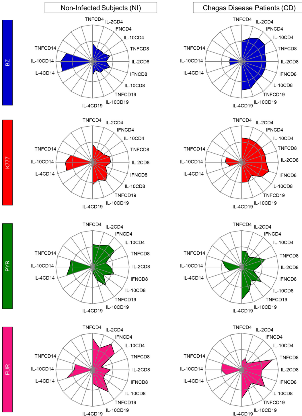
FIG 5 Drug-induced changes on in vitro intracytoplasmic cytokine signatures of innate and adaptive immunity. Radar graphs represent the balance of subjects with a high frequency of inflammatory (IL-2, TNF, IFN) or regulatory (IL-10, IL-4) cytokine-producing cells of innate (CD14) and adaptive (CD4, CD8, CD19) immunity. Graphs were constructed with each axis displaying the proportion of subjects with a high frequency of cytokine-producing cells within a given leukocyte subset. The values of each axis can be joined to form the central polygon area that represents the general inflammatory/regulatory cytokine balance. Increasing or decreasing central polygon areas reflect either higher or lower contributions, respectively, of the inflammatory versus regulatory cytokine balance in each group. Analysis of the radar chart axes highlights the contribution of a distinct leukocyte subset for the overall cytokine balance after treatment with BZ (blue), K777 (red), PYR (green), and FUR (pink) lead compounds. Groups were categorized as noninfected subjects (NI, n = 18 ) and Chagas disease patients (CD, n = 20 ).
