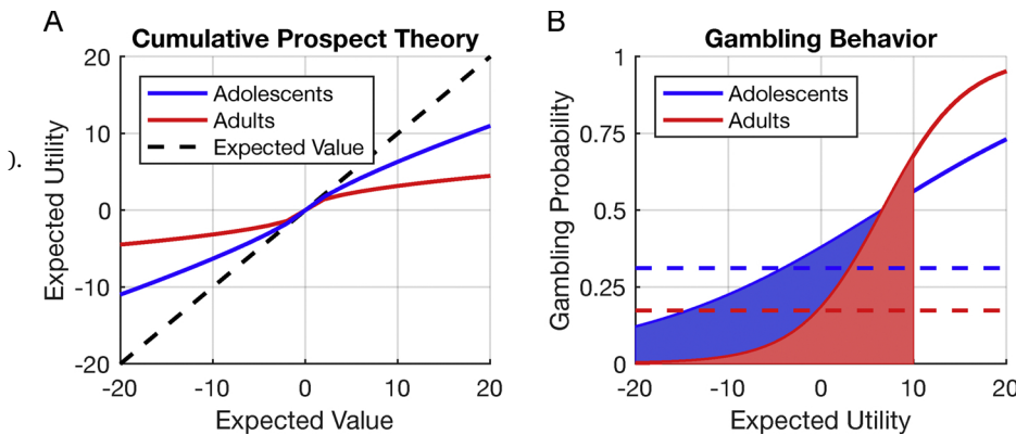
A) Fit of CPT for a set of choices by hypothetical adolescents and adults. B) Two response probability curves for two fictitious groups of adolescents and adults that only differ in their level of choice sensitivity (see Eq. (2) in text), but have the exact same EU estimations. Note that in this example the mean level of risky choices (as indicated with the dashed lines) will be higher for the adolescents than the adults.
