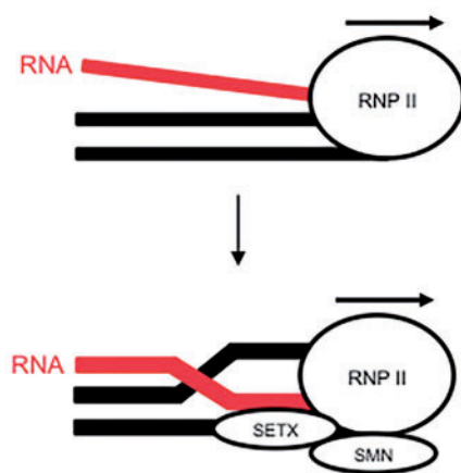
Figure 1 ALS-linked RNA processing factors are guardians of the genome. (A) Several factors associated with RNA processing, including FUS and TDP-43, are required to maintain R-loop homeostasis. Their depletion leads to R-loop-mediated genomic instability. (B) The resolution of R-loops involves the recruitment of the RNA/DNA helicase, SETX, which is recruited to R-loops by SMN - defects in either cause motor neuron cell death.
