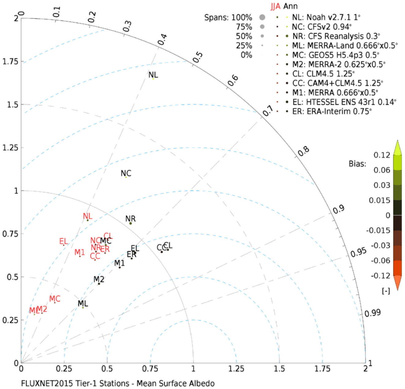
Figure 4. As in Fig. 3 for surface albedo; annual mean (black) and boreal summer (JJA) mean (red).
