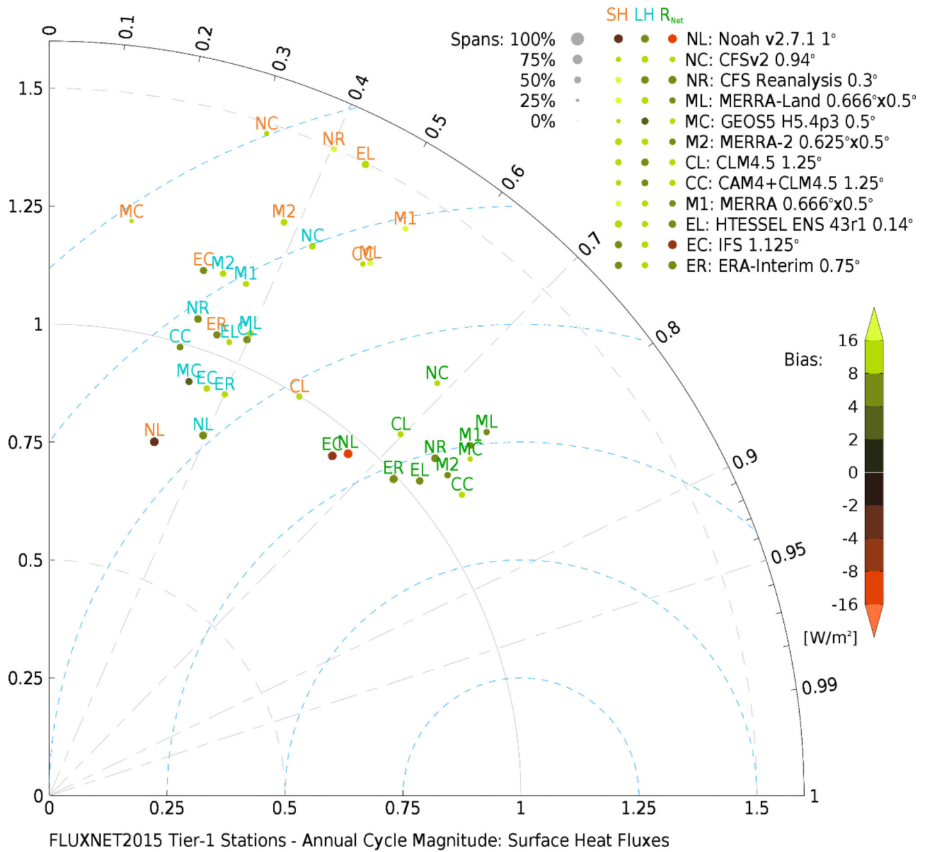
Figure 6. As in Fig. 3 for the magnitude of the annual cycle (first harmonic calculated from monthly means) of sensible heat flux (orange), latent heat flux (cyan) and net radiation at the surface (green).
