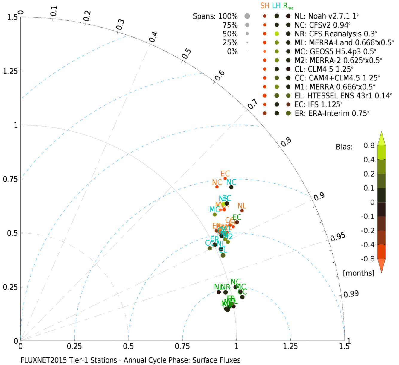
Figure 7. As in Fig. 6 for phase of the annual cycle of sensible heat flux (orange) and latent heat flux (cyan) and net radiation at the surface (green).
