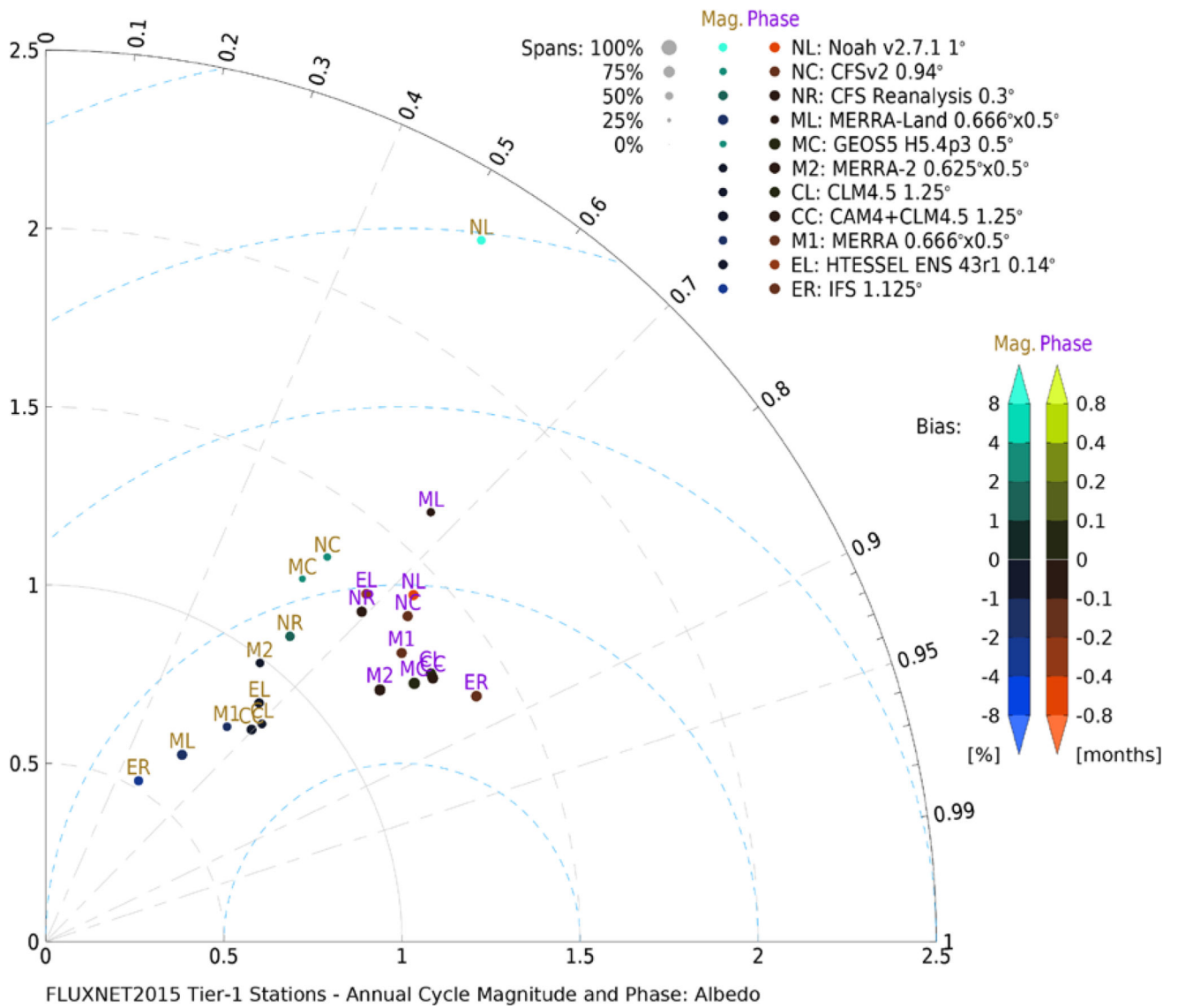
Figure 8. As in Fig. 6 for the magnitude (brown) and phase (purple) of the annual cycle of surface albedo.
