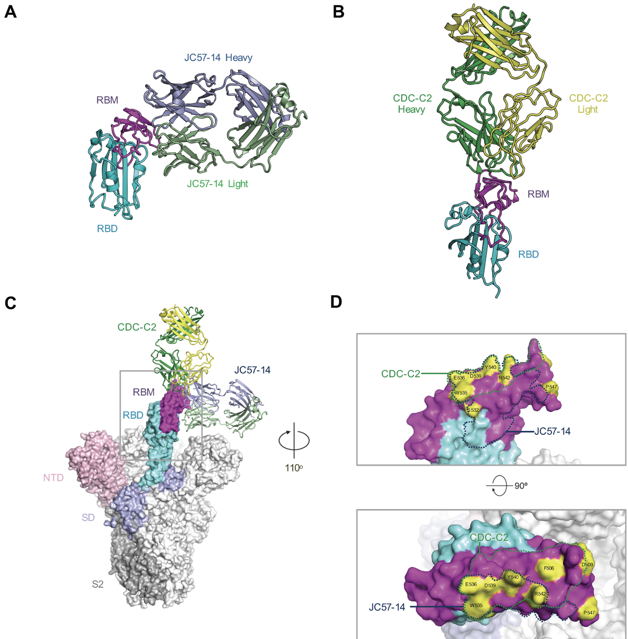
FIG 3 Structural characterization of macaque and human MERS virus-neutralizing antibodies. (A) Crystal structure of JC57-14 antibody bound to MERS England1 RBD. (B) Crystal structure of CDC-C2 bound to MERS England1 RBD. (C) JC57-14 and CDC-C2 are modeled using the MERS spike trimer structure (PDB code 5W9H) bound to a single RBD in the open conformation. (D) Antibody epitopes of JC57-14 and CDC-C2 are displayed on the surface of the RBD structure. Residues highlighted and labeled differing in natural viral variants were tested to characterize antibody epitopes.
