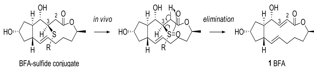
Scheme 5. Sulfoxide conjugate approach for BFA.
