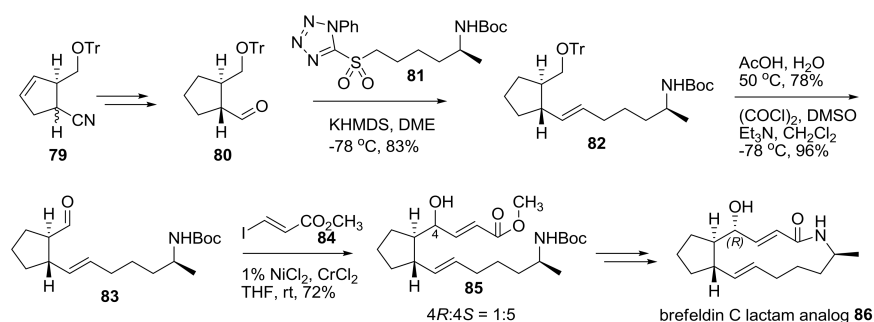
Scheme 17. Synthesis of brefeldin C lactam analogs. Tr: triphenylmethyl, KHMDS; Potassium bis(trimethylsilyl)amide, DME: dimethoxyethane, DMSO: dimethyl sulfoxide.
