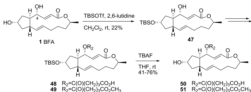
Scheme 10. Synthesis of 4-acyl BFA analogs. TBS: t -butyldimethylsilyl, Tf: trifluoromethanesulfonyl, TBAF: tetra- n -butylammonium fluoride.
