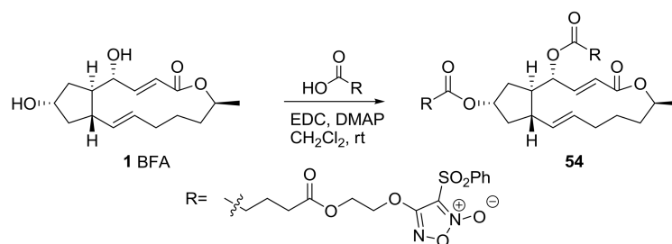
Scheme 12. Synthesis of NO-producing ester analogs of BFA.
