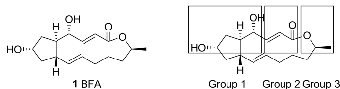
Figure 1. Structure of brefeldin A (BFA) and groups of its analogs based on structural modifications.
