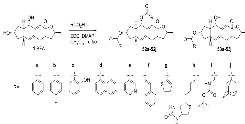
Scheme 11. Synthesis of BFA analogs with ester functional groups. EDC: 1-Ethyl-3-(3-dimethylaminopropyl)carbodiimide.
