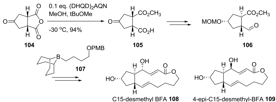
Scheme 22. Synthesis of C15-desmethyl BFA analogs. (DHQD) 2 AQN: Hydroquinidine (anthraquinone -1,4-diyl) diether.
