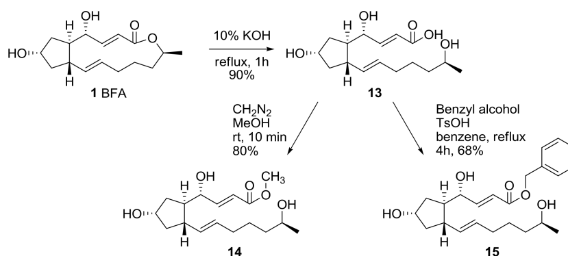
Scheme 4. Modification of the carbonyl group in BFA.
