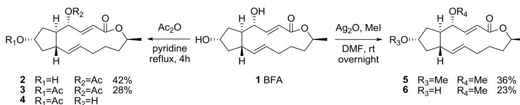
Scheme 1. Modification of the two hydroxyl groups in BFA. DMF: dimethylformamide.
