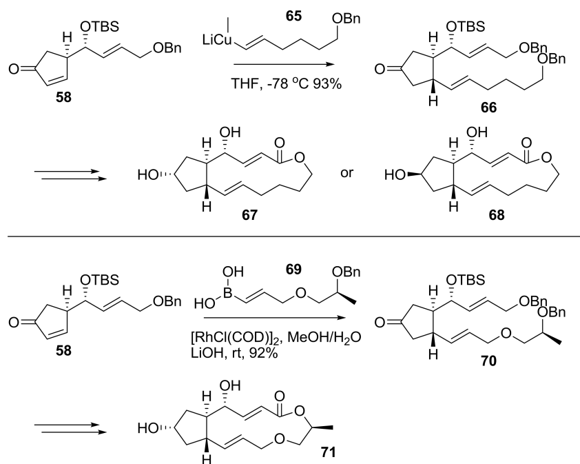
Scheme 15. Synthesis of NO-producing ester analogs of BFA. COD: cyclooctadiene.
