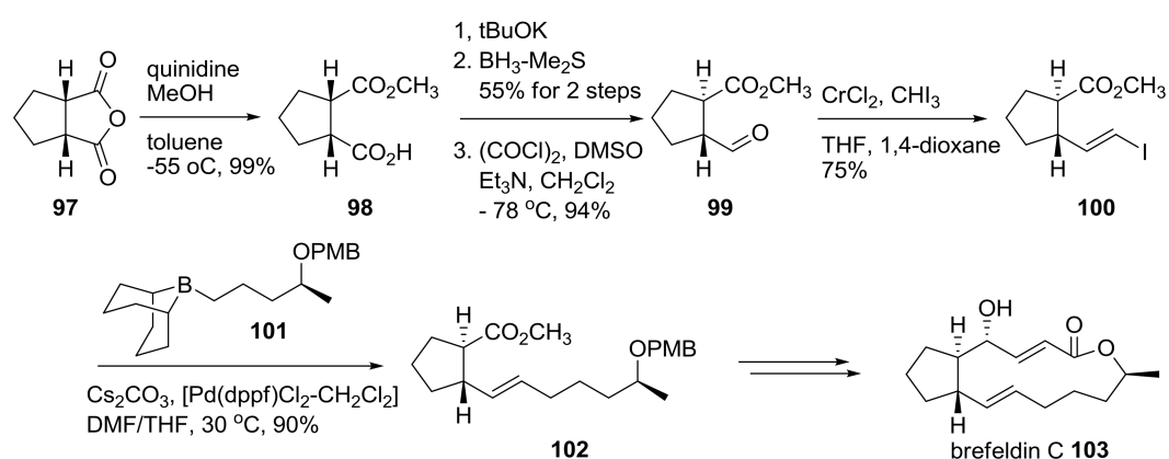
Scheme 21. Synthesis of brefeldin C and its analogs. PMB: para-methoxybenzyl; dppf: 1,1'-bis(diphenylphosphino)ferrocene.
