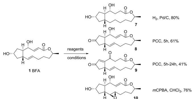
Scheme 2. Oxidation and reduction of BFA. PCC: pyridinium chlorochromate; m CPBA: meta -chloroperoxybenzoic acid.
