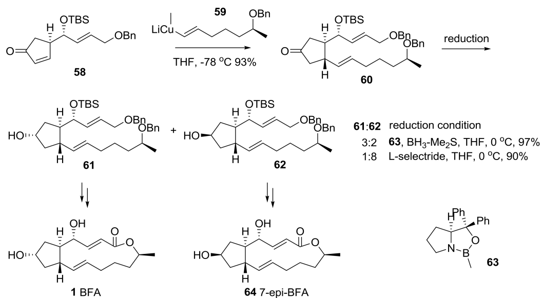
Scheme 14. Total synthesis of BFA and 7-epi-BFA using the conjugated addition route.
