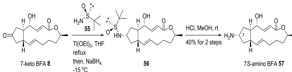
Scheme 13. Synthesis of 7-amino-BFA analogs.
