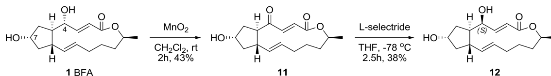
Scheme 3. Chiral inversion of the 4-hydroxyl group in BFA. L-selectride: lithium tri- sec -butyl(hydrido)borate; THF: tetrahydrofuran.
