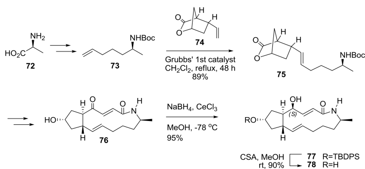
Scheme 16. Synthesis of 4- epi -BFA lactam analogs. Boc: t -butoxycarbonyl, CSA: camphorsulfonic acid, TBDPS: t -butyldiphenylsilyl.
