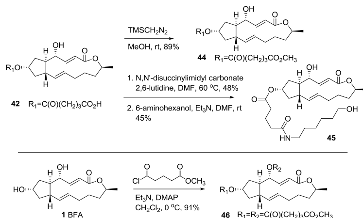
Scheme 9. Synthesis of BFA analogs with long lipid chains. TMS: trimethylsilyl; DMAP: 4-dimethylaminopyridine.
