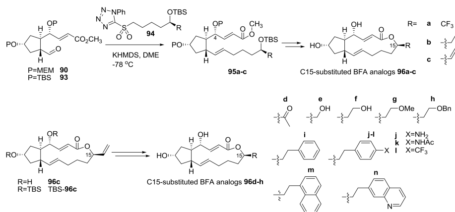
Scheme 20. Synthesis of C15-substituted BFA analogs.
