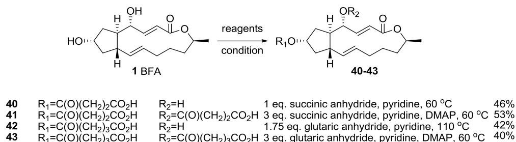
Scheme 8. Synthesis of succinyl or glutaryl BFA analogs.
