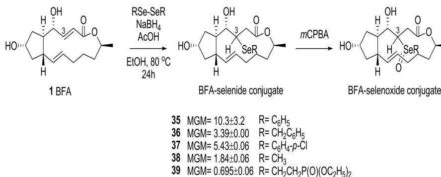
Scheme 7. Synthesis of selenide-conjugated BFA analogs and their MGMs.
