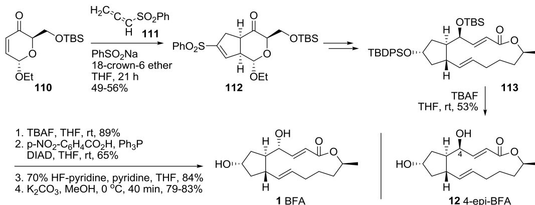
Scheme 23. Synthesis of BFA and its 4-epimer through cycloaddition of allenylsulfone strategy.
