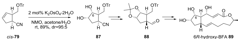
Scheme 18. Synthesis of (6R)-hydroxy-BFA analogs. NMO: N -methylmorpholine N -oxide.
