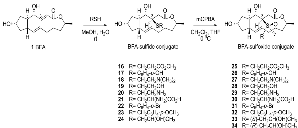
Scheme 6. Synthesis of sulfide- and sulfoxide-conjugated BFA analogs.
