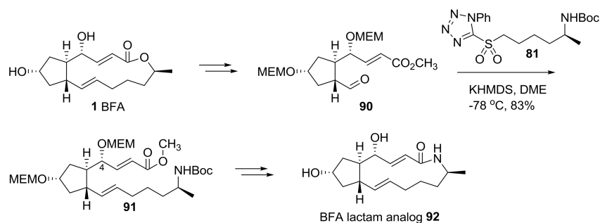
Scheme 19. Synthesis of BFA lactam analogs. MEM: 2-methoxyethoxymethyl.
