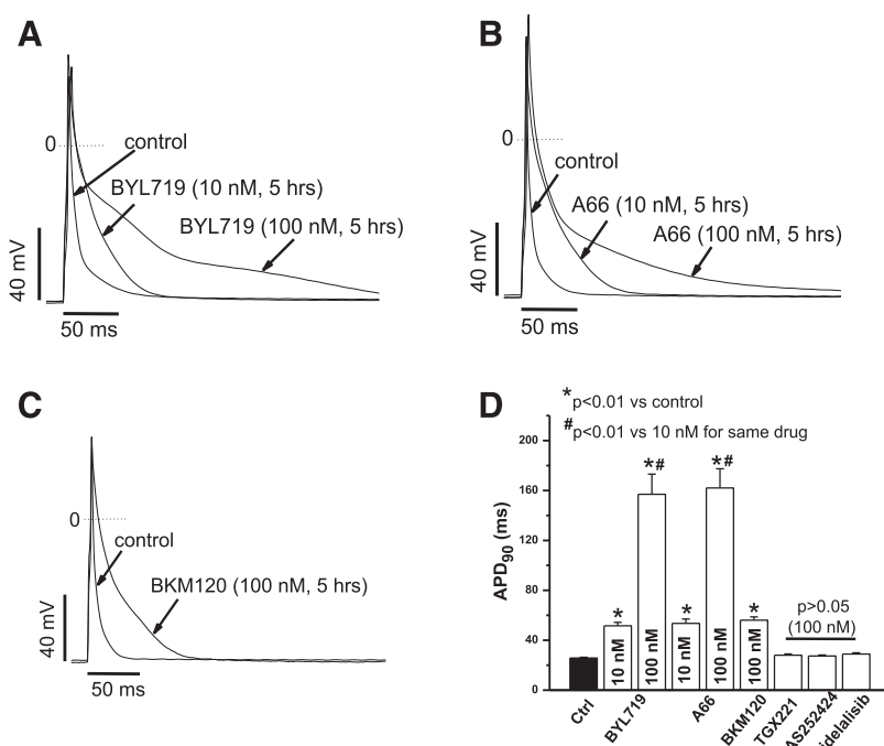
Fig. 1. Chronic PI3K- \alpha and pan-PI3K inhibitors caused action potential prolongation and abnormal APs in adult mouse ventricular myocytes. (A) Chronic BYL719 (5 hours) prolonged APs in a concentration-dependent manner at a stimulation rate of 1 Hz. (B) Chronic A66 (5 hours) prolonged APs in a concentration-dependent manner at a stimulation rate of 1 Hz. (C) Chronic the pan-PI3K inhibitor BKM120 (5 hours) prolonged AP at a stimulation rate of 1 Hz. (D) Summary of the effects on APD 90 by all inhibitors at 1 Hz ( n = 5-8 each).
