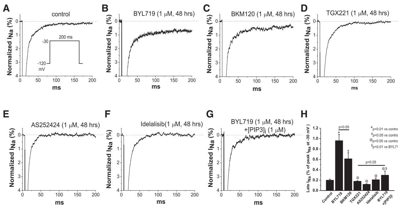
Fig. 4. Chronic PI3K- \alpha and pan-PI3K inhibitors increased late I_{Na} in SCN5A -transfected CHO cells. (A) Control I_{Na} recorded with the protocol shown. (B) Current trace showing that chronic PI3K- \alpha inhibitor BYL719 increased late I_{Na} . (C) Current traces showing that chronic pan-PI3K inhibitor BKM120 increased late I_{Na} . (C-F) Current traces showing that the inhibitors targeting PI3K- \beta , - \gamma , and - \delta did not alter late I_{Na} . (G) Current trace showing that internally adding PIP3 antagonized chronic BYL719-increased late I_{Na} . (H) Summary ( n = 6-8 each group).
