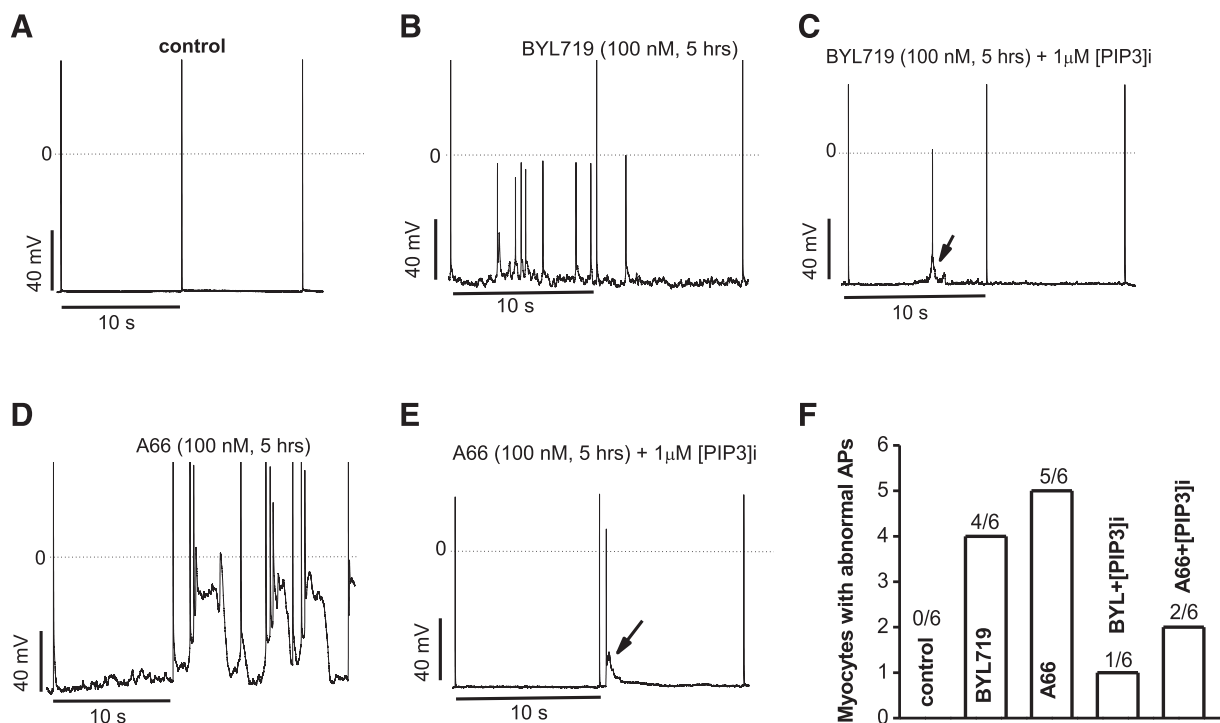
Fig. 2. Internally applied PIP3 antagonized action potential abnormalities by chronic PI3K- \alpha inhibitors in adult mouse ventricular myocytes. (A) Control AP traces at a stimulation rate of 0.1 Hz. (B) Chronic BYL719 induced triggered activity. (C) Inclusion of PIP3 in the internal pipette solution dramatically attenuated BYL719-induced abnormal action potentials (arrow). (D) Chronic A66 caused triggered activity. (E) Inclusion of PIP3 in the internal pipette solution dramatically attenuated A66-induced abnormal action potentials (arrow). (F) Summary of the numbers of myocytes with abnormal APs in each group.
