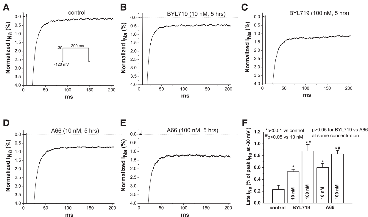
Fig. 3. Chronic PI3K- \alpha inhibitors increased late I_{Na} in adult mouse ventricular myocytes. (A) control current traces recorded with the protocol shown. (B and C) Effects of two concentrations of BYL719 (10 and 100 nM) on late I_{Na} after 5-hour treatment. (D and E) Effects of two concentrations of A66 (10 and 100 nM) on late I_{Na} after 5-hour treatment. (F) Summary of the concentration-dependent increases in cardiac late I_{Na} in mice by the two inhibitors ( n = 6-7 each group). The two inhibitors increased late I_{NaL} to the same extent.
