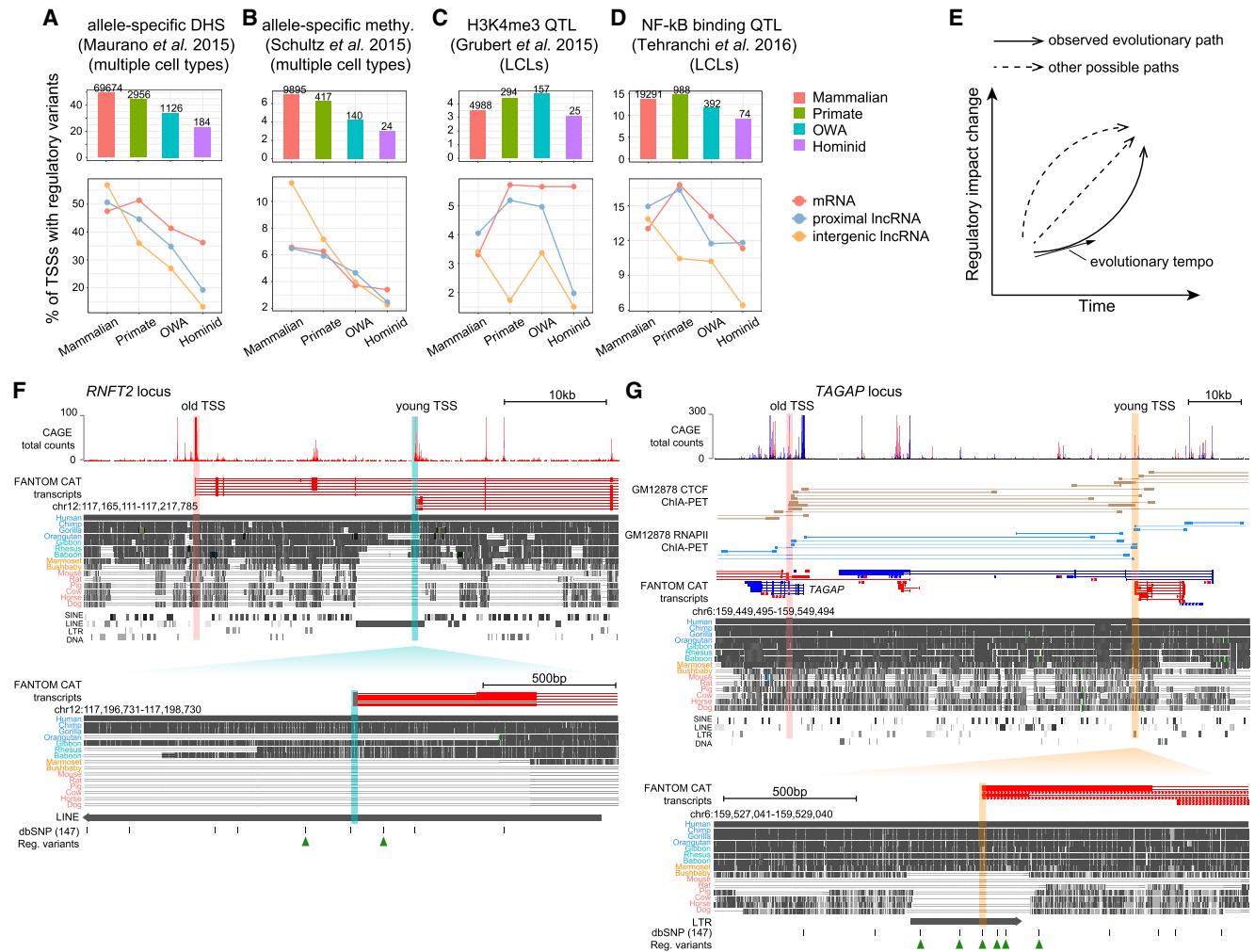
Figure 5. Temporal and spatial constraints on the regulatory evolution of young TSSs. (A) (Top) Proportion of TSSs harboring regulatory variants associated with allele-specific DHS within TSS \pm 1 kb for each TSS group; numbers above bars indicate the numbers of TSSs with regulatory variants. (Bottom) Proportions of TSSs harboring regulatory variants in different TSS subgroups, defined by transcript type. (B) Proportion of TSSs harboring regulatory variants associated with allele-specific methylation within TSS \pm 1 kb. (C) Proportion of TSSs harboring H3K4me3 QTLs within TSS \pm 1 kb. Data generated from lymphoblastoid cell lines (LCLs). (D) Proportion of TSSs harboring NF-kB complex binding (RELA ChIP) QTLs within TSS \pm 1 kb. (E) Schematic illustration depicting different possible paths for regulatory evolution of young TSSs. (F) Genome browser view of a young TSS cis -proximal to old TSSs. (Top) FANTOM CAT transcript models (red for forward-strand, blue for reverse-strand); genomic alignments and TE annotations obtained from the UCSC Genome Browser. (Bottom) Enlarged region of an "OWA" TSS inside a LINE element. Beneath the alignments are the common SNPs (allele frequency \geq 0.01 ) from dbSNP database and SNPs associated with regulatory variation. (G) A young TSS trans -proximal to old TSSs. (Top) Similar to F but with additional CTCF and RNAP II ChIA-PET data for GM12878 cell line. (Bottom) Enlarged region of the young TSS. Below the alignments are the common SNPs (allele frequency \geq 0.01 ) and regulatory variants.
