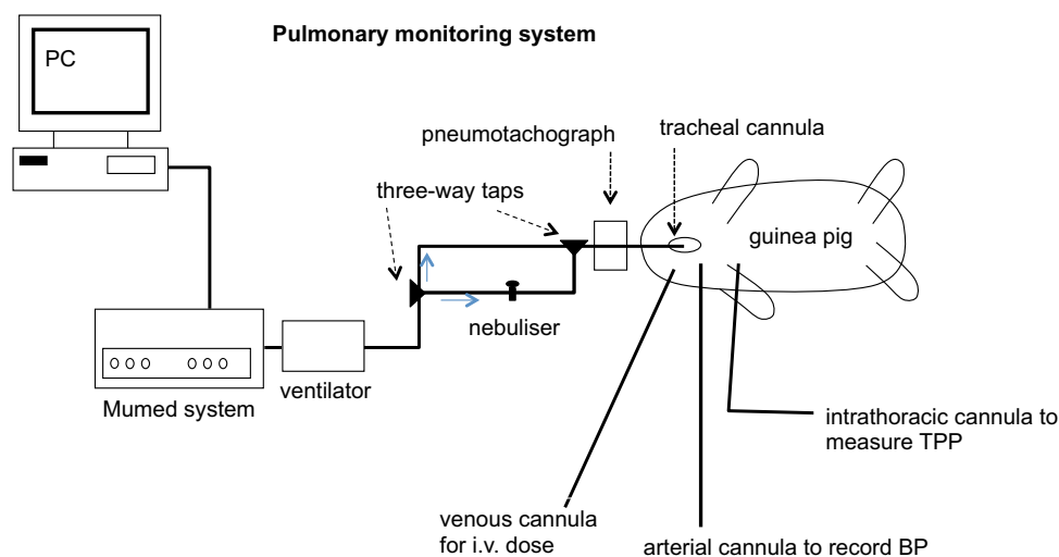
Fig. 3 Schematic presentation of the integrated experimental setup for ventilation, nebulised aerosol administration and measurement of the pulmonary function of the guinea pigs. BP blood pressure, TPP transpulmonary pressure
