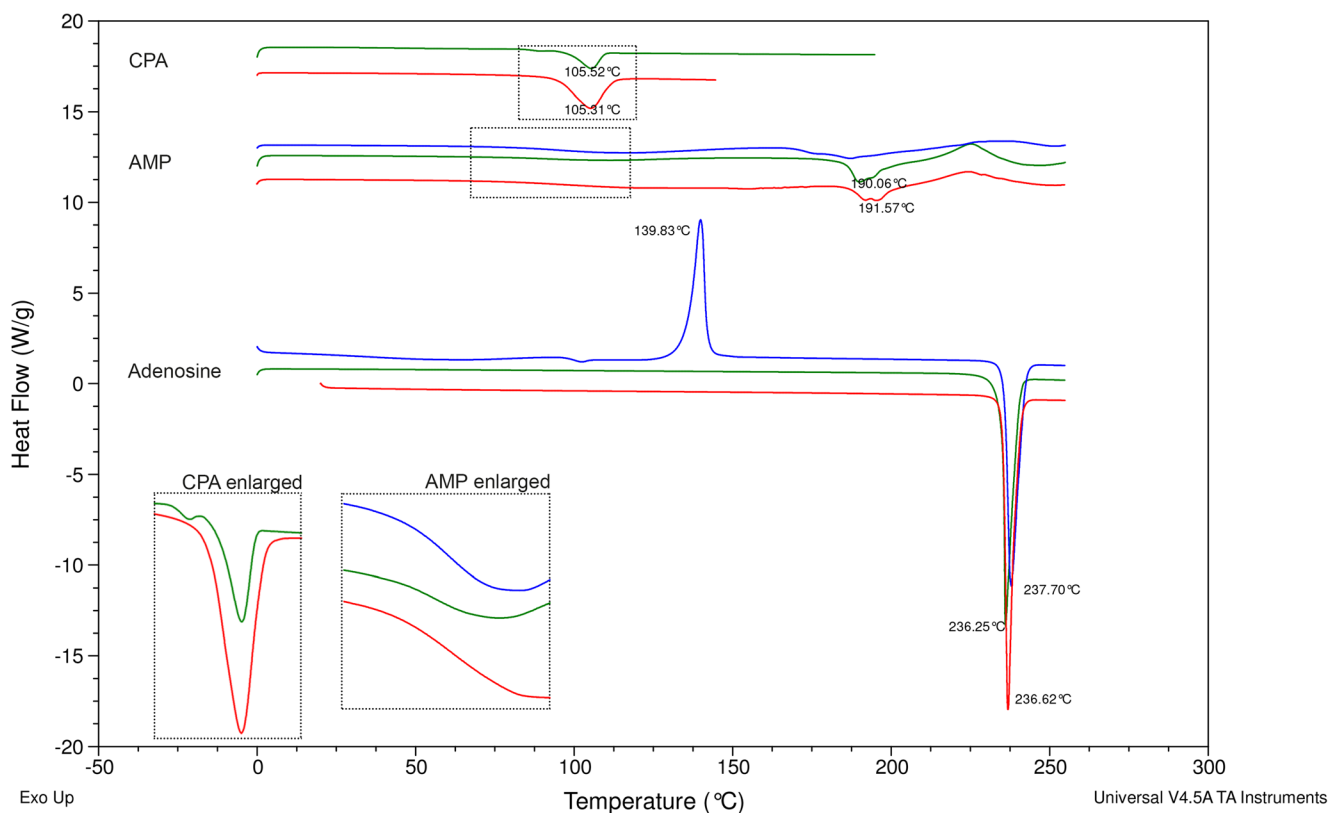
Fig. 4 Differential scanning calorimetry thermograms of adenosine, adenosine 5'-monophosphate (AMP) and N 6 -cyclopentyladenosine (CPA) starting materials (red) and after micronisation (green) or spray drying (blue). Offset on the y-axis has been used for presentation purposes and clarity
