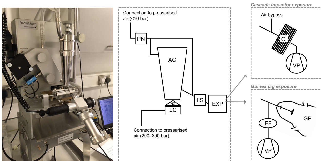
Fig. 1 The PreciseInhale system. A powder dose is loaded into the loading chamber, which is then pushed through the nozzle by a high-pressure air jet into the aerosol chamber, where it subsequently settles by opposing force of gravity. It is then released towards the exposure module, for which the flow is created by a vacuum pump. A light-scattering device measures the particle density in the aerosol, which is used to track the emitted dose. The exposure modules used in this study were a Marple cascade impactor and intracheally intubated guinea pigs.
