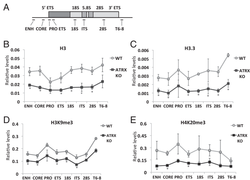
Fig. 3. rDNA chromatin state is changed in ATRX KO cells. (A) A schematic diagram of the rDNA cluster, showing the locations of various PCR fragments across the region. (B and C) ChIP/qPCR analyses of H3 (B) and H3.3 (C) in WT and ATRX KO (clone KO #1) mouse ES cells showing substantial losses of H3 and H3.3 at the rDNA repeats in the absence of ATRX. (D and E) To determine the levels of heterochromatin present at the rDNA repeats, H3K9me3 (D) and H4K20me3 (E) ChIP/qPCR analyses were performed and normalized to the H3 ChIP/qPCR values, and reductions in both heterochromatin marks, H3K9me3 and H4K20me3, appeared to be significant at a subset of the rDNA repeat loci (error bars represent SD, n = 4 , *P < 0.05 ).
