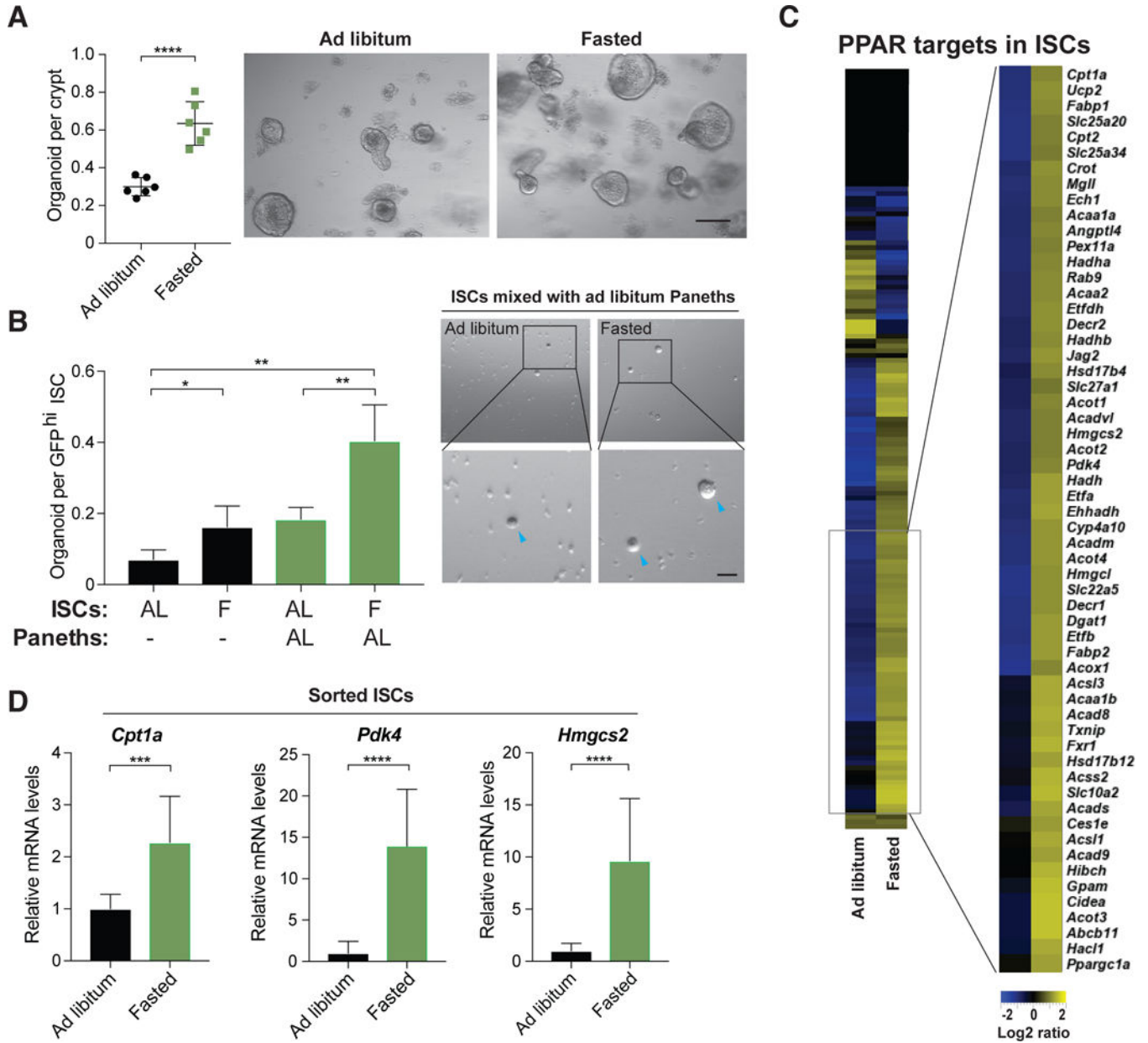
Figure 1. Fasting induces fatty acid oxidation and improves intestinal stem cell function (A) Organoid frequency of crypts from 10-12 week old ad libitum or 24-hour fasted mice. Representative images of crypt culture from each condition. n=6 mice per group. (B) ISCs from 24-hour fasted animals (F) had significantly enhanced organoid-forming capacity when mixed with age matched Paneth cells from ad libitum (AL) mice. Blue arrowheads indicate organoids. n=3 mice per group. (C) Heat map of RNA-Seq analysis showing log 2 -transformed relative expression of PPAR target genes in ISCs (Lgr5-GFP hi ) from AL or 24 hour fasted mice. (D) qRT-PCR analysis confirming PPAR target gene induction in ISCs (Lgr5-GFP hi ) following a 24 hour fast. \beta actin was used as a housekeeping gene. n=7 mice.
