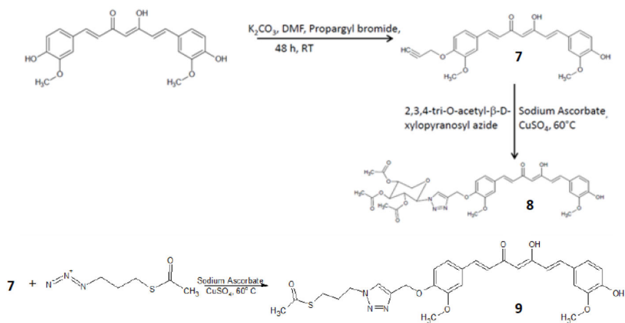
Scheme 2. Synthesis of Curcumin click chemistry analogues
