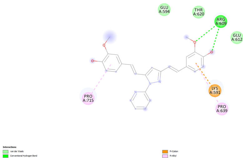
Figure 4. (a). Predicted binding mode of pyrazole compound 2 in the active site of STAT3-SH2. (b). 2-D interaction diagram
