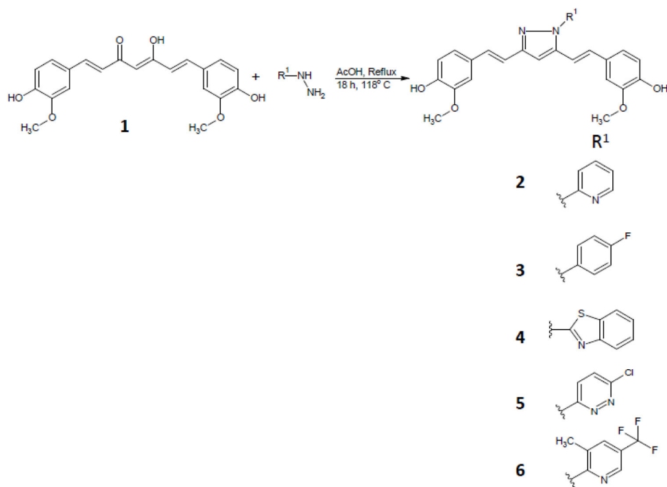
Scheme 1. Synthesis of Curcumin pyrazole analogues.
