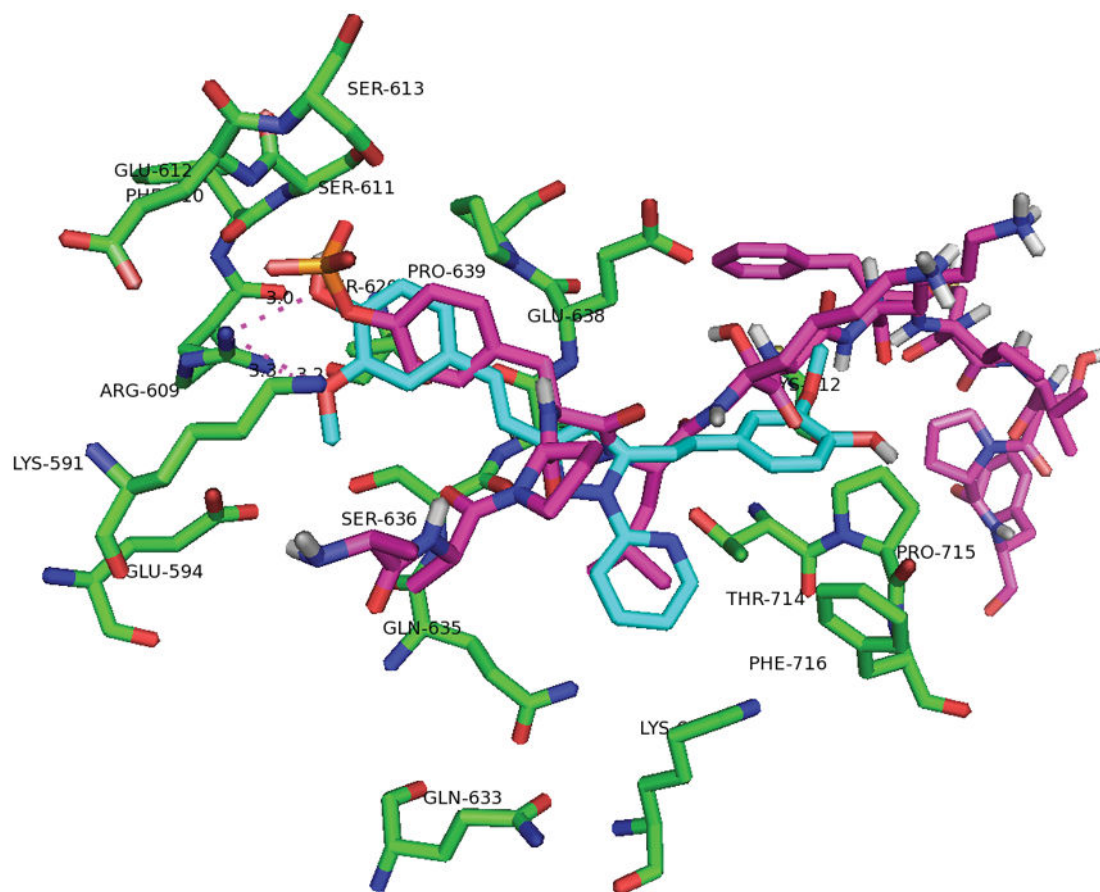
Figure 5. Overlay of phosphor-tyrosine peptide (magenta) and pyrazole compound 2 (cyan).
