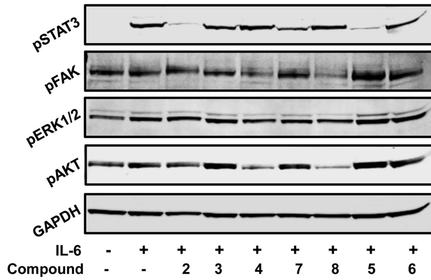
Figure 3. Effect of curcumin analogues on pSTAT3, pFAK, pERK1/2 and pAKT signaling pathways at IC 50 dose level.
