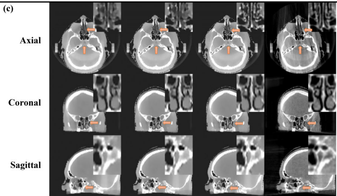
Figure 9. Comparisons of brain CBCT reconstructed via TV, EPTV and PCTV using a) 41 projections, b) 50 projection and c) 62 projections. Full sampling FDK using 500 projections are listed at the right column as the reference. Zooming in images are listed in the right and upper corner.
