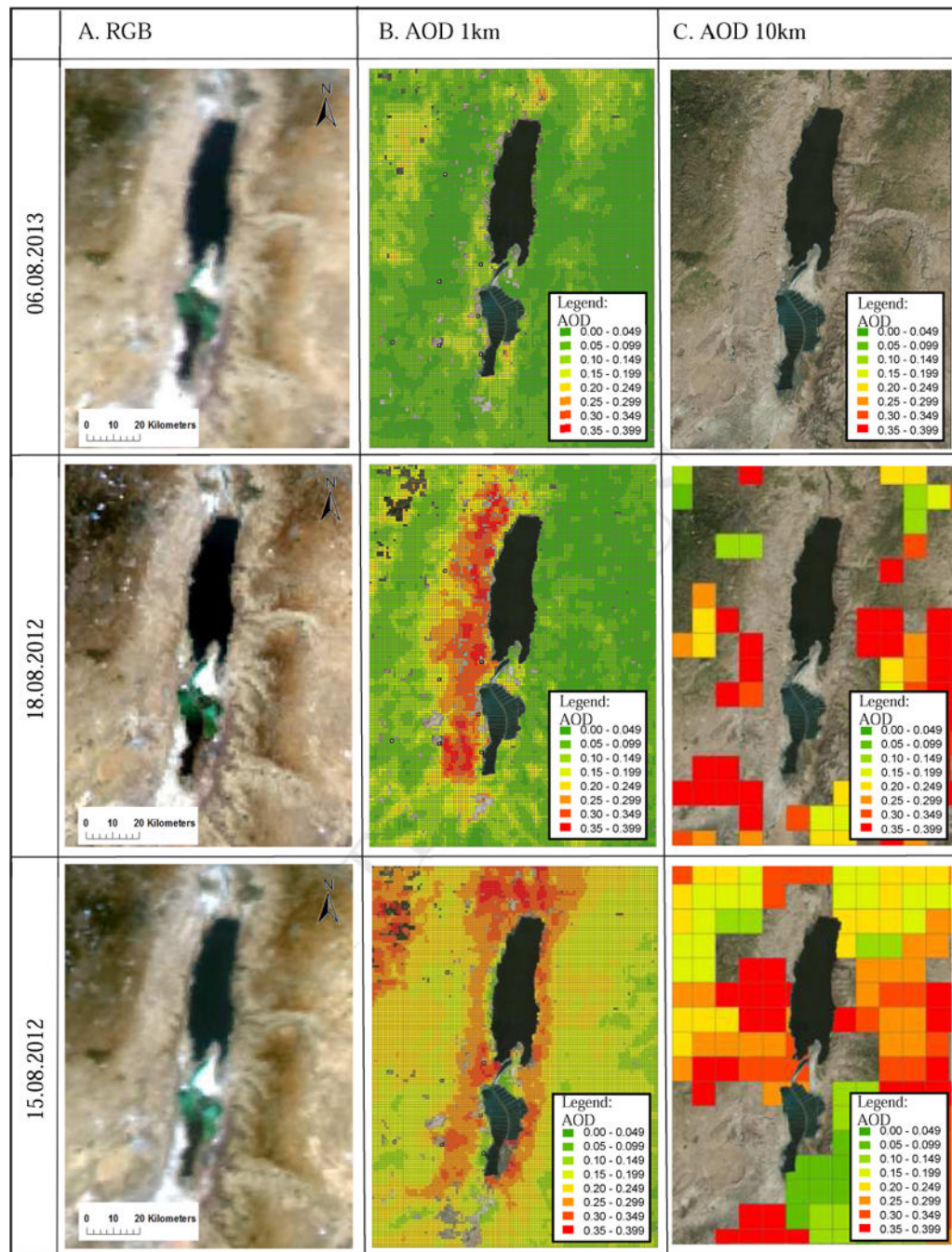
Figure 1. AOD for selected days in August above the Dead Sea region. Panel A shows RGB data; Panel B shows MAIAC AOD data at a 1km resolution; and Panel C shows MODIS Collection 6 combined (Dark Target + Deep Blue) AOD product. Note missing AOD values when compared to MAIAC.
