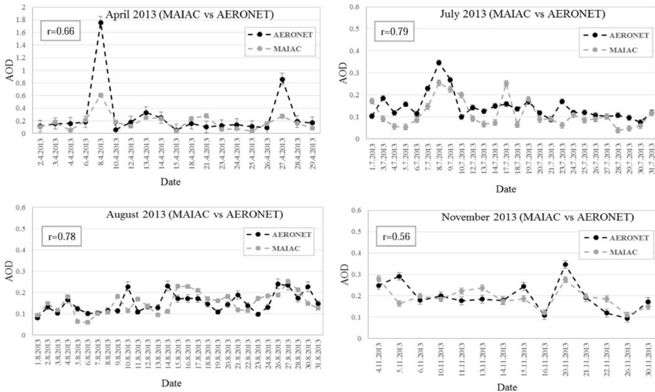
Figure 4. Monthly trend of AOD for Sde Boker: Comparison between AERONET and MAIAC AOD retrievals. Error bars represent standard deviation.
