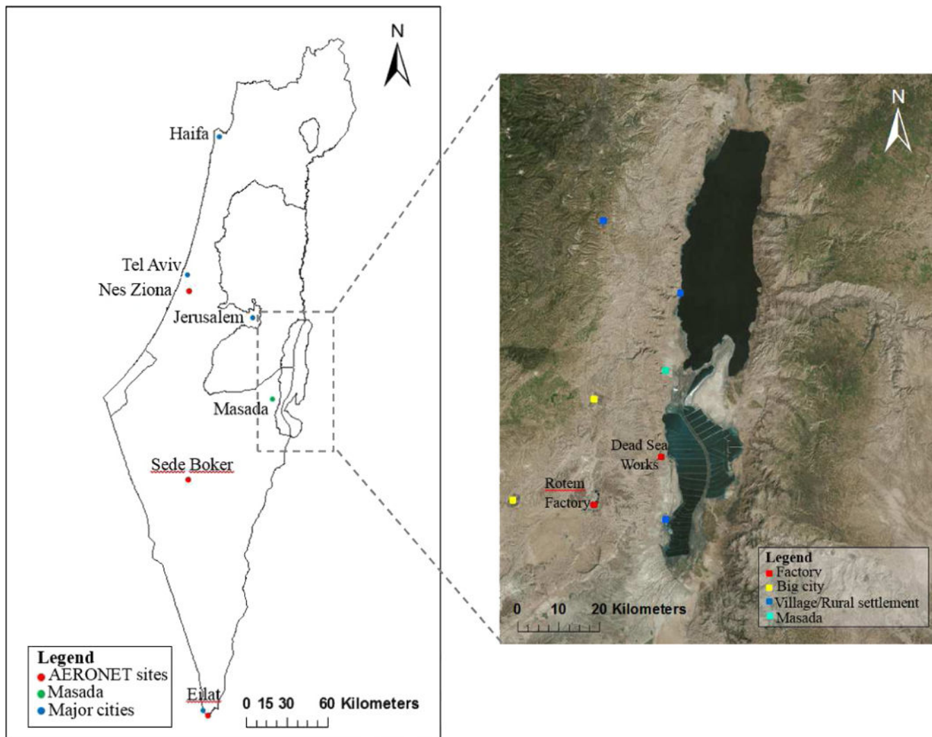
Figure 2. Study Area. Left: a map of the area of Israel, with the Dead Sea region highlighted by the dotted line (major cities, AERONET stations, and Masada historical site marked); Right: an enlargement of the study area (rural settlements, cities, and industrial zones marked). The historical site of Masada is also marked.
