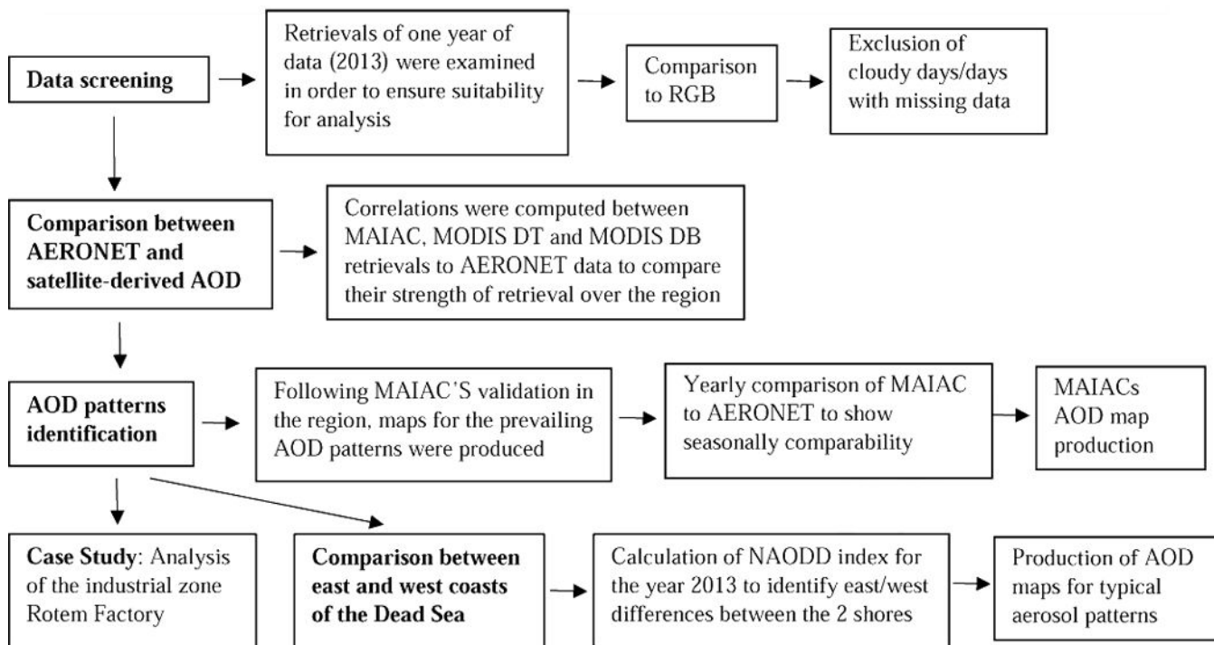
Figure 3. Flow chart of the data analysis process.
