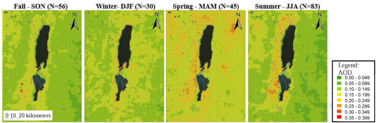
Figure 5. Seasonal average of MAIAC AOD for 2013 (where N represents the number of available days for analysis in each season).
