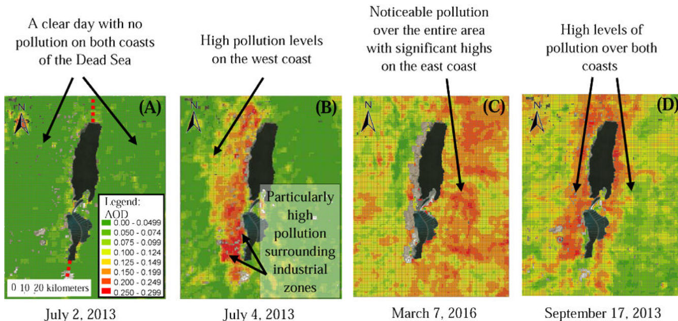
Figure 6. AOD for selected days in above the Dead Sea region, each one representative of a different typical AOD pattern: (A) A clear day with hardly any aerosols over the region, on July 2, 2013 (the dotted line represents the division between the eastern and western parts of the Dead Sea region); (B) High AOD values concentrated along the west coast only (on July 4, 2013); (C) High AOD on the eastern side of the Dead Sea (March 7, 2016); and (D) elevated levels of aerosols above the entire region, with significantly higher aerosols concentration surrounding both eastern and western coasts of the Dead Sea (on the September 17, 2013).
