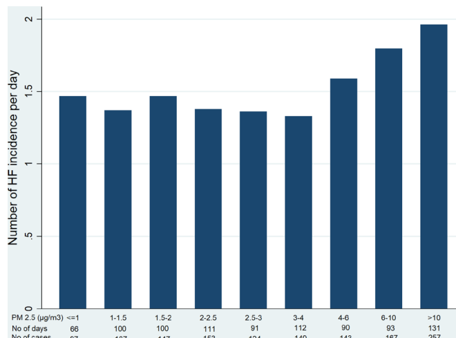
Figure 7 Possible threshold of PM_{2.5} with heart failure (HF) incidence.
