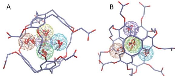
Fig. 7 Water map clustering for hexa-acid cryptophane m3n3 . (A) Side view and (B) top view differ by a rotation of 90^\circ . Five position-based water clusters are indicated by wireframe spheres with radius of 1 Å and are colored in order of decreasing population: orange, yellow, tan, green and purple. Within each cluster, coordinates of six representative water molecules (red) are rendered.
