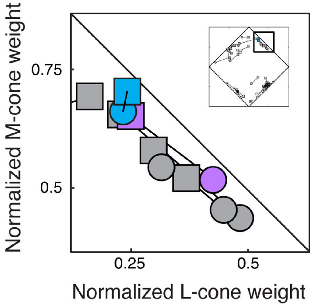
Figure 5. Normalized cone weight estimates for the example neuron from Figure 1 estimated via the response-weighted average (purple) and maximum likelihood (blue). Normalized cone weight estimates derived from the phosphor noise (squares) agreed closely with those derived from the cone noise (circles) using both techniques.
