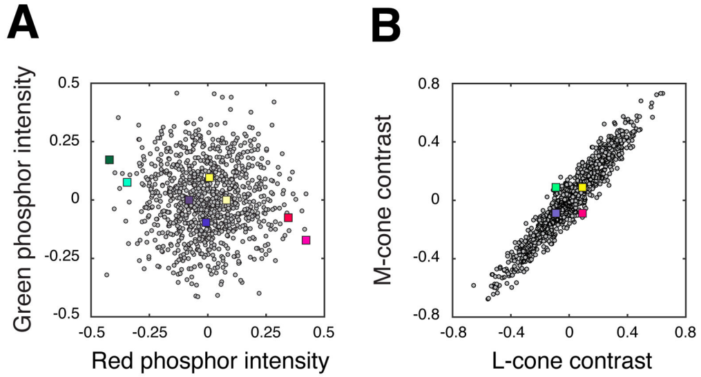
Figure 3. Phosphor noise stimuli (gray circles) and cone noise stimuli (colored squares) represented in two color spaces. (a) Phosphor and cone noise stimulus distributions projected onto the red-green plane of phosphor space. The phosphor noise distribution is approximately radially symmetric (RS) in this space, and the cone noise distribution is distended. (b) The same two distributions projected onto the LM plane of cone space. In this color space, the cone noise distribution is approximately RS, and the phosphor noise distribution is distended. Only four colored squares are visible because +S- and -S-cone stimuli have an equal projection onto this plane.
