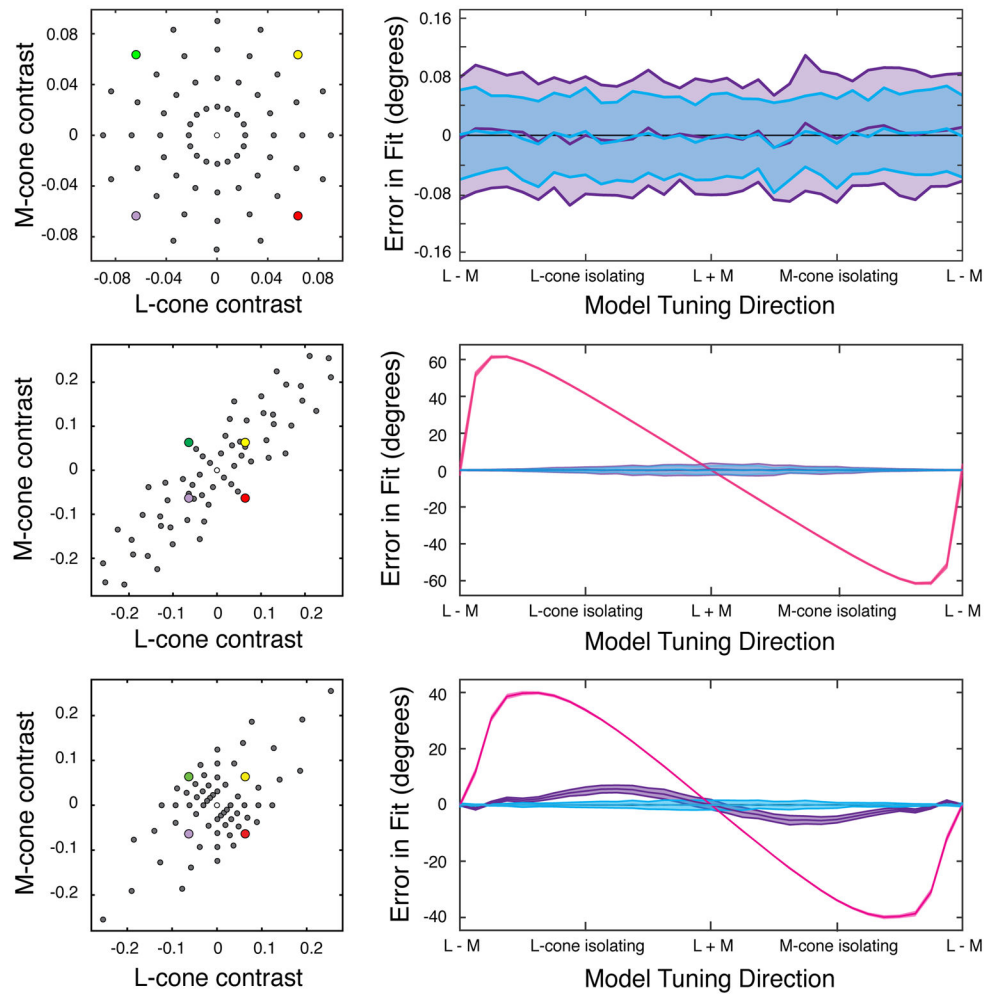
Figure 6. Estimates of preferred color direction obtained from the responses of simulated neurons. Preferred color directions were estimated with three techniques and three stimulus distributions. Gray circles represent stimuli that were presented to the simulated neuron. The purple, green, yellow, and red points represent identical lights in each distribution. For simplicity, only L- and M-cone modulations were simulated. (a) Left: a radially symmetric stimulus distribution. Right: the mean and standard deviation of the error between the true and estimated preferred directions. Estimation via the response-weighted average stimulus (RWA) (purple) and maximum likelihood (blue) were both unbiased. (b) Left: a distended stimulus distribution that was RS when whitened. Right: estimation via the RWA of the non-whitened distribution (pink) was biased, but estimation via linear regression (purple) and maximum likelihood (blue) were unbiased. (c) Left: a distended stimulus distribution that could not be made RS by linear transformation. Right: estimation via the RWA (pink) and linear regression (purple) were both biased, but estimation via maximum likelihood (blue) remained unbiased.
