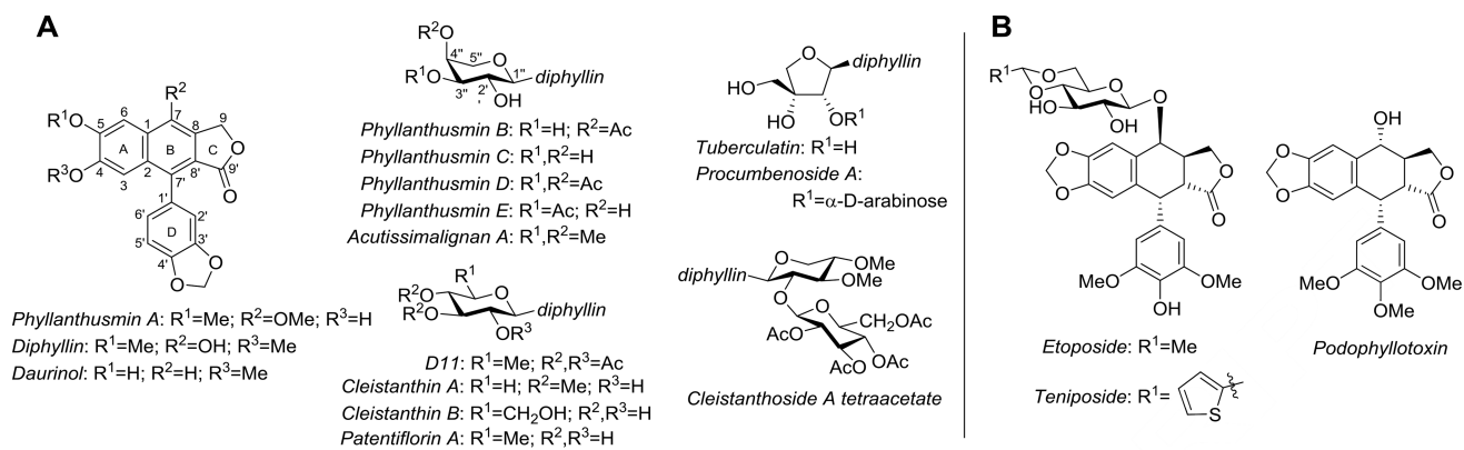
Figure 1. Phyllanthusmins A–E along with structurally related arlynaphthalene lignan lactones (A) and aryletralin lignan lactones (B).
