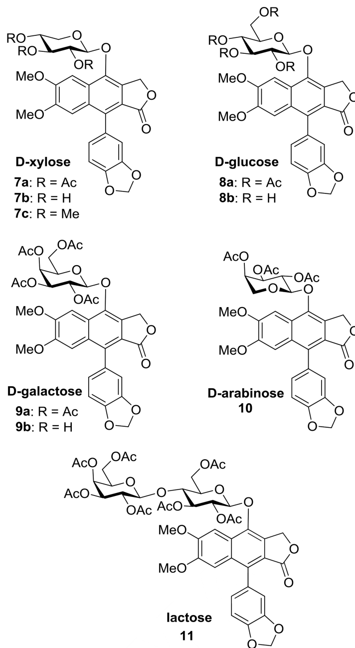
Figure 2. Chemical structures of compounds 7–11.
