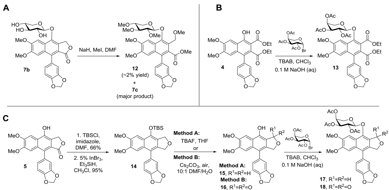
Scheme 2. Preparation of C-ring lactone analogues 12 , 13 , 17 , and 18 .
