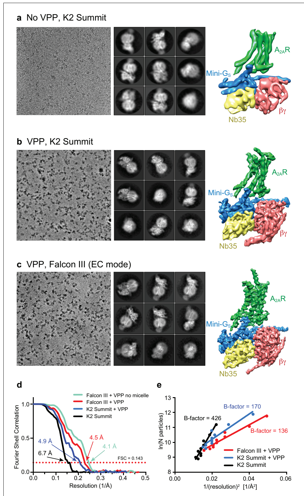
Figure 2. Cryo-EM of the A_{2A}R complex in the presence and absence of a VPP. (a-c) Each panel contains three sections, with the left-hand section showing a representative micrograph obtained on a Titan Krios, the central section depicting 2D class averages and the right-hand section the refined 3D reconstruction obtained from the data collected. (a) Data collected without using a VPP on a K2 Summit detector. (b) Data collected using a VPP on Figure 2 continued on next page
