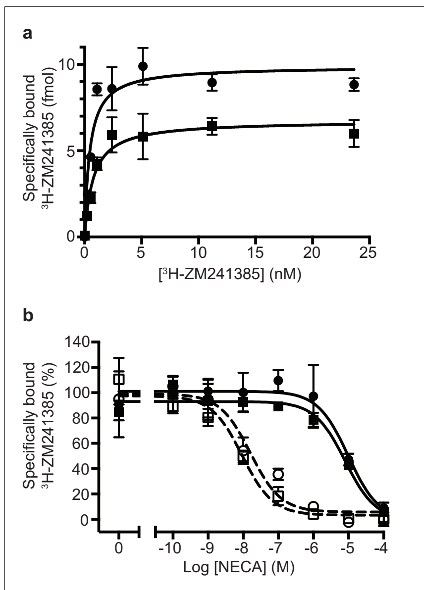
Figure 1. Pharmacological analyses of A_{2A}R . (a) Saturation binding of the inverse agonist ^3\text{H-ZM241385} to A_{2A}R constructs gave the following apparent K_D s: A_{2A}R (circles), 0.5 \pm 0.1 nM; \text{TrxA-A}_{2A}R (squares), 0.8 \pm 0.2 nM. (b) Competition binding curves measuring the displacement of ^3\text{H-ZM241385} with increasing concentrations of NECA gave the following K_i s for NECA; A_{2A}R (filled circles), 1.0 \pm 0.5 \mu\text{M} ; A_{2A}R + \text{mini-G}_5 (open circles, dashed line), 2.6 \pm 1.8 nM; \text{TrxA-A}_{2A}R (filled squares), 1.1 \pm 0.4 \mu\text{M} ; \text{TrxA-A}_{2A}R + \text{mini-G}_5 (open squares, dashed line), 1.8 \pm 1.2 nM. Data plotted are the average from two independent experiments performed in duplicate with error bars shown as the SD.
