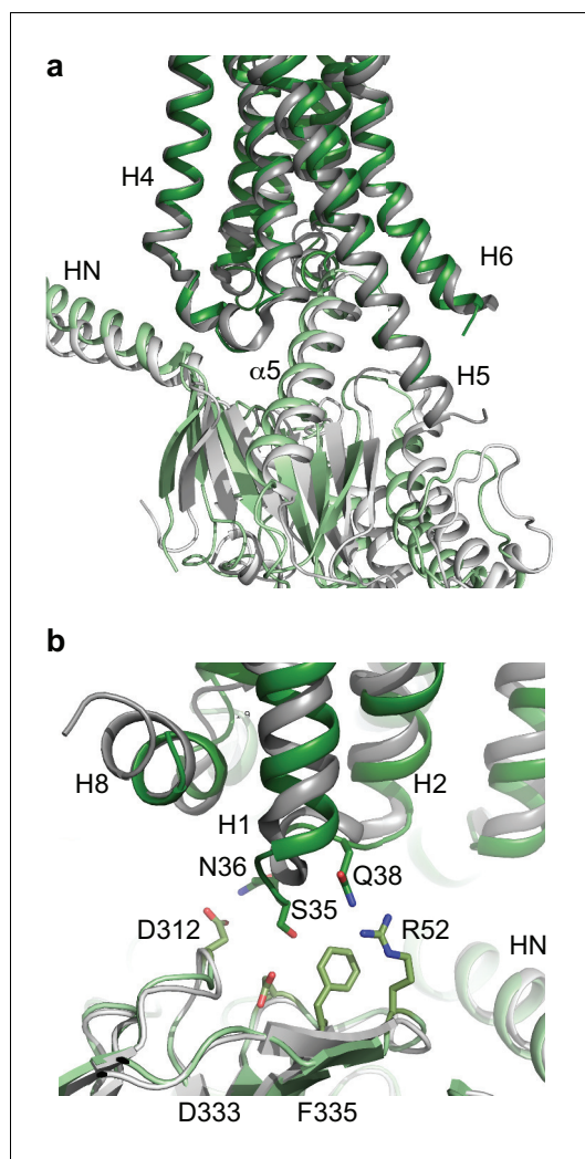
Figure 7. Comparison of A_{2A}R and \beta_2AR coupled to heterotrimeric G_s . (a) A_{2A}R (dark green) and \beta_2AR (dark grey) were aligned using regions of the receptors predicted to be within the cytoplasmic leaflet of the lipid bilayer. The position of mini- G_s (pale green) coupled to A_{2A}R is compared to the position of the GTPase domain of the \alpha subunit (pale grey) coupled to \beta_2AR . The \beta\gamma subunits and Nb35 have been omitted for clarity. (b) Transmembrane region H1 and ECL1 in A_{2A}R (dark green) extends closer to the \beta subunit (pale green), whereas \beta_2AR (dark grey) is too far away from the \beta subunit (pale grey) to make extensive contacts. DOI: https://doi.org/10.7554/eLife.35946.010
