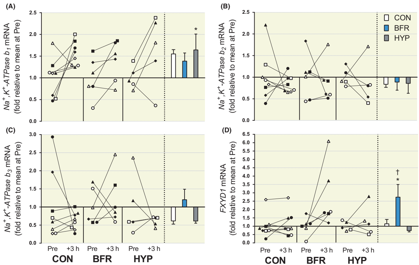
FIGURE 2 NKA- \beta -isoform and FXDY1 mRNA responses to moderate-intensity interval running performed without or with blood flow restriction or in systemic hypoxia. (A) \beta_1 , (B) \beta_2 , (C) \beta_3 and (D) FXDY1, mRNA content. Individual changes from before (Pre) to 3 hours after exercise (+3 hours) are displayed on the left with each symbol representing one participant across trials and figures. On the right are bars representing mean ( \pm SEM) changes relative to Pre for exercise alone (CON, white; n = 8 ), with blood flow restriction (BFR, blue; n = 6 ) or in systemic hypoxia (HYP, grey; n = 5 ). * P < .05 , different from Pre
