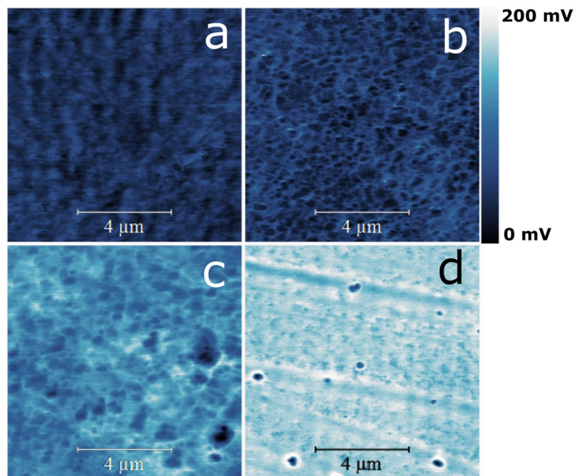
Figure 9. Kelvin probe force microscopy (KPFM) surface potential maps ( 10 \times 10 \mu\text{m}^2 ) of samples (a) [\text{Cu}]/[\text{Te}] = 1.25 , (b) [\text{Cu}]/[\text{Te}] = 1.5 , (c) [\text{Cu}]/[\text{Te}] = 1.75 and (d) [\text{Cu}]/[\text{Te}] = 2 .
