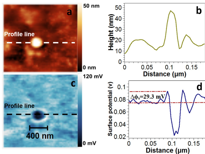
Figure 10. Representative images of the [\text{Cu}]/[\text{Te}] = 2.0 film obtained by AFM and KPFM of a crystal cluster. (a) Topographic image obtained on tapping mode. (b) Height profile of the indicated line. (c) Surface potential distribution. (d) Surface potential profile along the indicated line.
