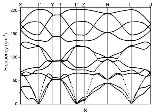
Figure 2. Phonon dispersion curves of CuTe (vulcanite).
