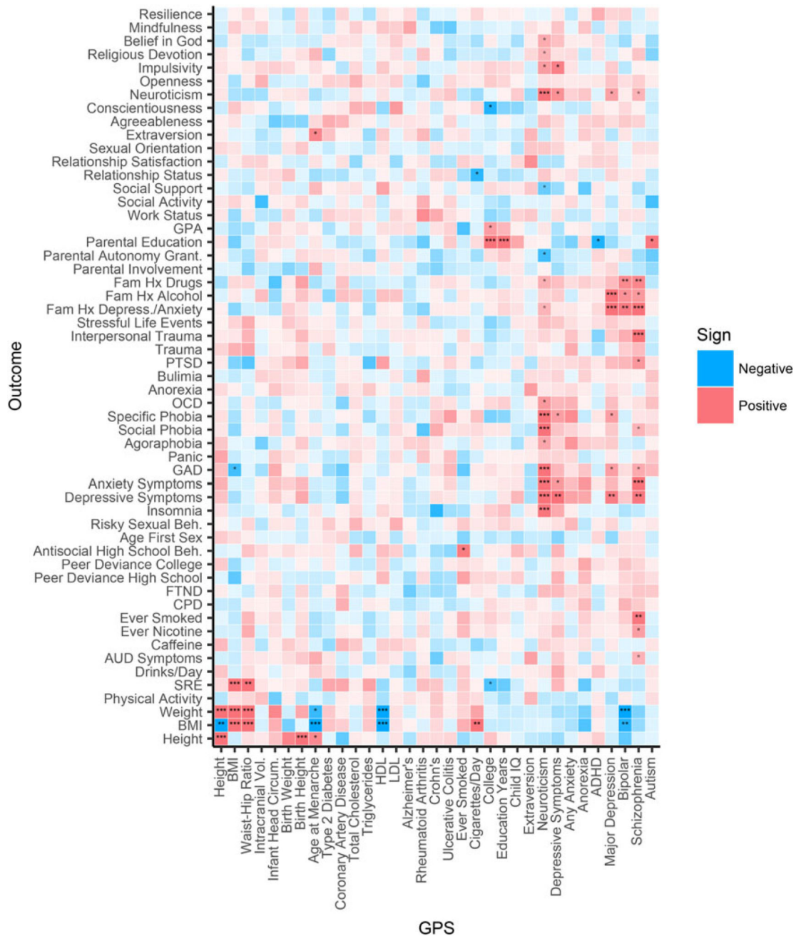
Fig. 2. Phenome on GPS regression q -values in European Sample (EUR). GPS displayed with prior proportion of causal effects = 0.3. Here, asterisks in the cells of the heatmap denote results of greater effect: *** = q -value < 0.01, ** = q -value < 0.05, * = q -value < 0.16. Blue values reflect a negative association, and red reflect positive association. Intensity of color indicates -\log_{10} p value.
