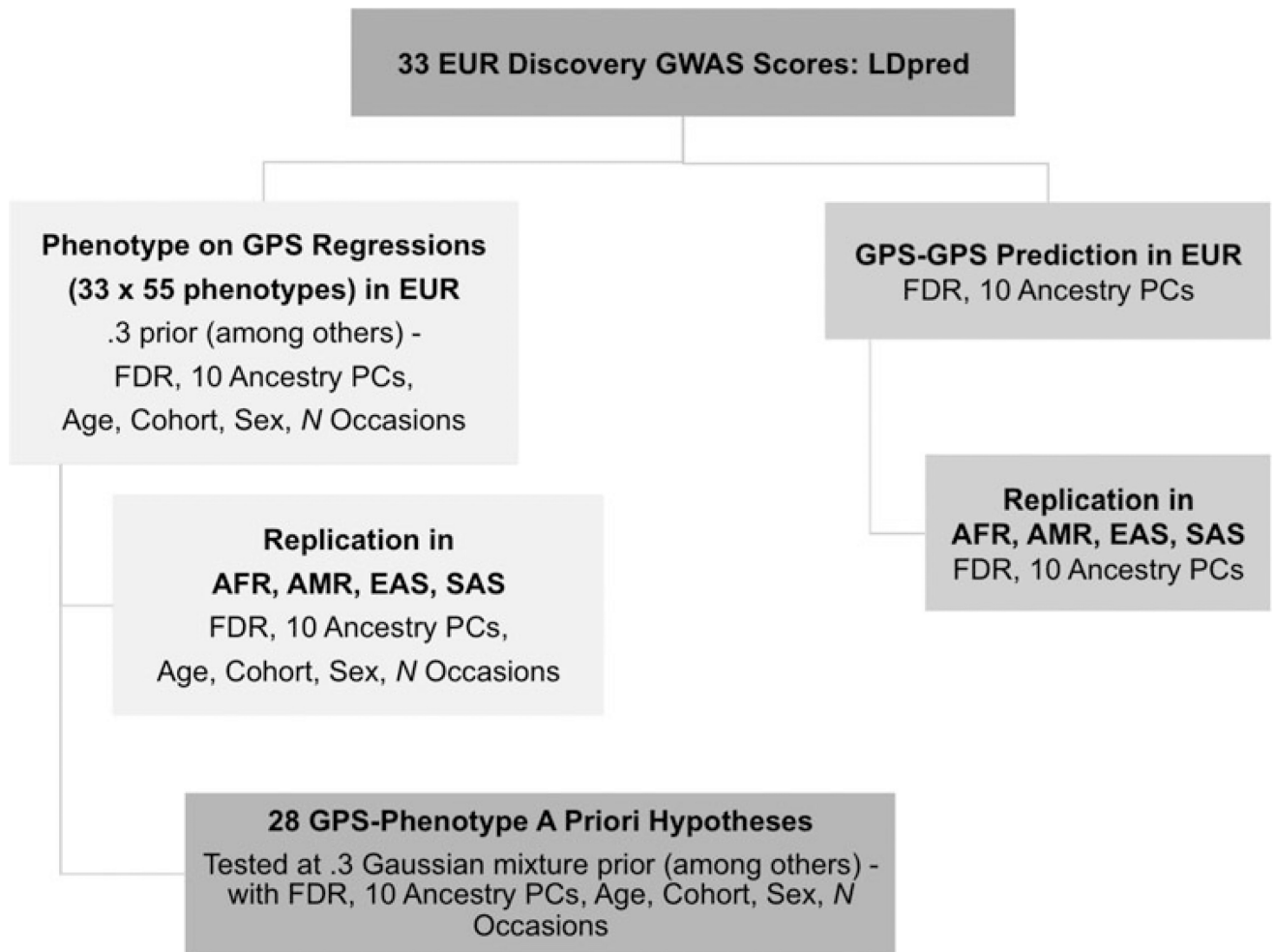
Fig. 1. Flow chart of the GPS-phenome and GPS-GPS analyses. GWAS, genome wide association study; FDR, false discovery rate; GPS, genome-wide polygenic score; PC, principal component.
