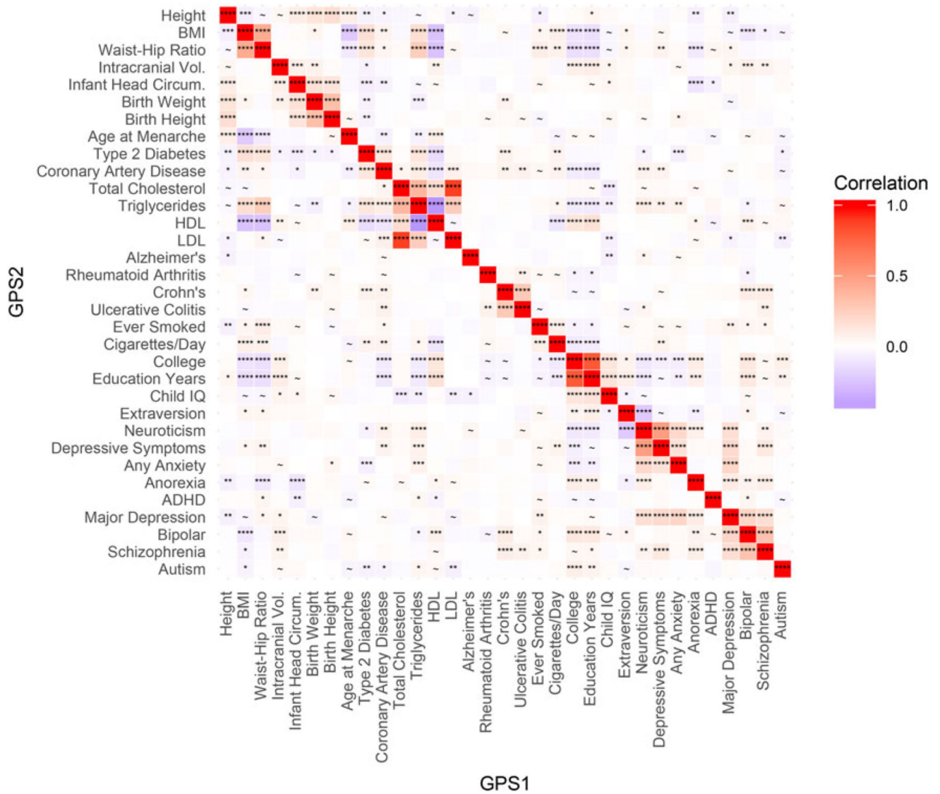
Fig. 3. Genetic Overlap and Co-Heritability of GPS in European Sample (EUR). Heatmap of partial correlation coefficients between GPS with prior proportion of causal effects = 0.3. Here, asterisks in the cells of the heatmap denote results of greater effect: **** = q -value < 0.0001, *** = q -value < 0.001, ** = q value < 0.01, * = q value < 0.05, and ~ = suggestive significance at q value < 0.16. Blue values reflect a negative correlation, and red reflect positive correlation.
