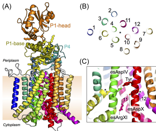
Figure 2. (A) The crystal structure of SecDF in the I form (PDB ID: 5XAP). SecDF consists of 12 TMs (TM1, blue; TM2, pale blue; TM3, turquoise; TM4, green; TM5, greenish yellow; TM6, pale greenish yellow; TM7, yellow; TM8, pale orange; TM9, orange; TM10, red; TM11, deep pink; and TM12, magenta), P1-base (yellow), P1-head (orange), and P4 (cyan) domains. Side chains of the highly conserved regions D1, D3, D5, F1 and F2 are depicted as stick representations. (B) TM region of SecDF cross-sectioned at the middle of the membrane and viewed from the periplasm. The asterisk shows the pseudosymmetrical center. The TM numbers are shown. (C) The important area in the center of the TM region. The essential, conserved residues, esAspIV, esAspX and esArgXI, are shown as stick representations. The important Tyr is located near the esAspIV. The corresponding positions of the inactive mutants of EcSecDF (Nouwen and Driessen 2005) in TM6 and TM12 are also shown as stick representations and indicated by asterisks.
