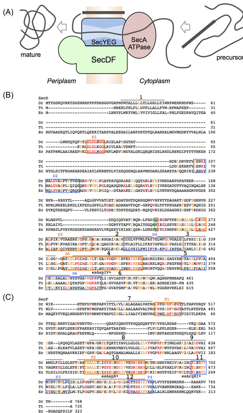
Figure 1. (A) Bacterial protein translocation across the membrane. SecA and SecDF drive protein translocation via the SecYEG complex, a protein conducting channel. (B) Sequence alignment of SecD from Deinococcus radiodurans (Dr), Thermus thermophilus (Tt) and Escherichia coli (Ec). (C) Sequence alignments of SecF from Dr, Tt and Ec. The TM numbers are shown. Perfectly and highly conserved residues (Furukawa et al. 2017) are colored red and orange, respectively. Essential residues Asp in TM4 (esAspIV), Asp in TM10 (esAspX) and Arg in TM11 (esArgXI) are indicated by solid circles. The conserved regions D1-6 and F1-4 (Eichler 2003) are highlighted by colored squares. The green box indicates EcSecD R407 and its corresponding residues (see also Fig. 5).
