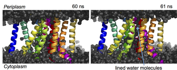
Figure 4. Snapshots of the MD simulation at 60 and 61 ns with dehydration of esAspIV. The water molecules queue from the cytoplasm to the periplasm through the TM region at 61 ns.
