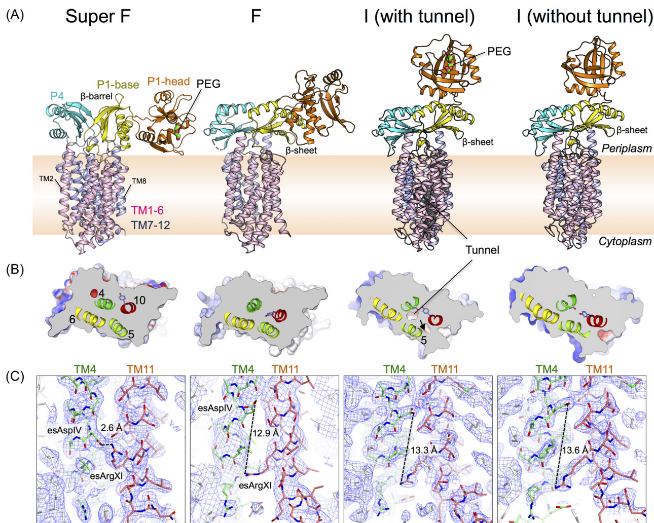
Figure 3. Crystal structures of SecDF. (A) The overall structures of the Super F, F, I (with tunnel) and I (without tunnel) forms (PDB ID: 3AQF, 5YHF, 5XAN-Mol B, and 5XAN-Mol A, respectively). PEG molecules in the periplasmic cavity are shown by stick representations. (B) Cut-away models of the surface representations of the middle TM regions viewed from the periplasm. Displacement of TM5 creates a tunnel. The important Tyr and esAspIV are shown by stick representations. (C) Electron density maps of SecDF. The 2F_o - F_c electron density maps in the Super F form (contoured at 1.0 \sigma ), F form (contoured at 1.5 \sigma ), and I form (contoured at 1.5 \sigma ). The esAspIV and esArgXI residues are labeled. Distance between the OD2 of esAspIV and NH2 of esArgXI are shown.
