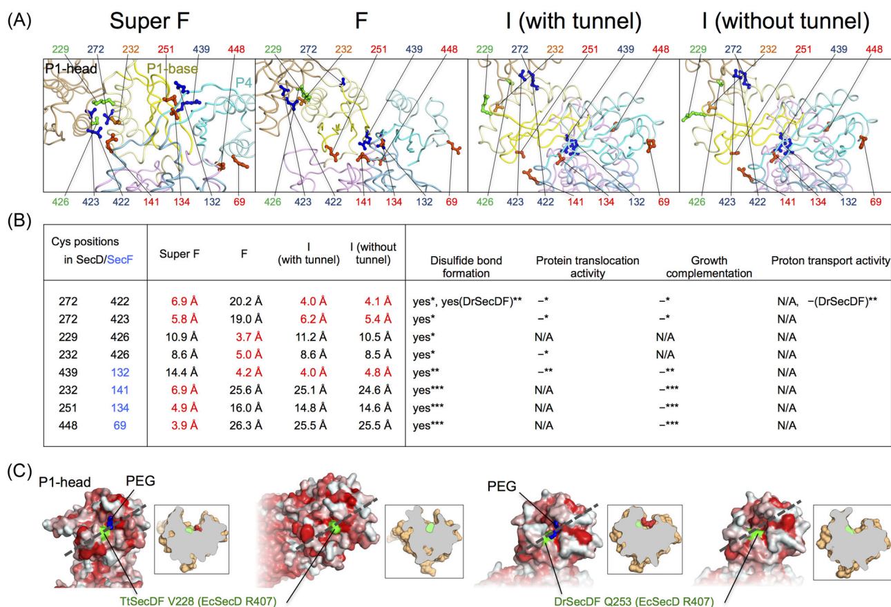
Figure 5. Flexibility of the periplasmic region. (A) Close up views of the periplasmic domain of SecDF (color scheme same as in Fig. 3A). The substituted corresponding positions of double cysteine mutants of EcSecDF are shown by the ball and stick model. (B) Summary of previous functional analyses of the EcSecDF mutants. The distance between the C \beta atoms of the substituted positions of SecD (black) and SecF (blue), protein translocation activity, growth complementation, and proton transport activity of the double cysteine mutants in disulfide bond form are summarized *(Tsukazaki et al. 2011); ** (Furukawa et al. 2017); *** (Furukawa et al. 2018). -: inactive, N/A: not available. C, P1-head cavities. Surface representation (left) colored according to hydrophobicity, from white (hydrophilic) to red (hydrophobic). The corresponding residue of EcSecD R407 interacting with precursor is colored green and indicated in Fig. 1. PEG molecules in the cavity are shown by stick representations. Cut-away models (right) of the surface representations along the dotted line.
