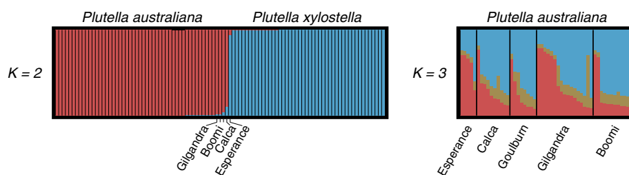
Fig. 5 Proportional assignment of Plutella individuals to genotypic clusters, K , based on STRUCTURE analysis. Individuals are represented by vertical bars and genotypic clusters are represented by different colors. Left panel: Analysis at K = 2 for 52 P. australiana and 47 P. xylostella individuals sorted left-to right by proportion of cluster membership. The predominantly red bars correspond to P. australiana individuals and the predominantly blue bars correspond to P. xylostella individuals identified through mtDNA genotypes. Locations are labelled for five individuals showing > 1% genotypic admixture. Right panel: Analysis at K = 3 for 52 P. australiana individuals sorted left-to-right by proportion of cluster membership within geographic locations, showing a high degree of genotypic admixture among individuals across locations
