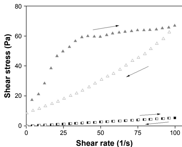
Figure 2 Rheograms of formulations F (squares) and F100 (triangles). Notes: Ascendant curve, filled symbols; descendent curve, empty symbols. F is the liquid crystal system; F100 is a 1:1 (wt/wt) dilution of F containing 100% artificial saliva.
