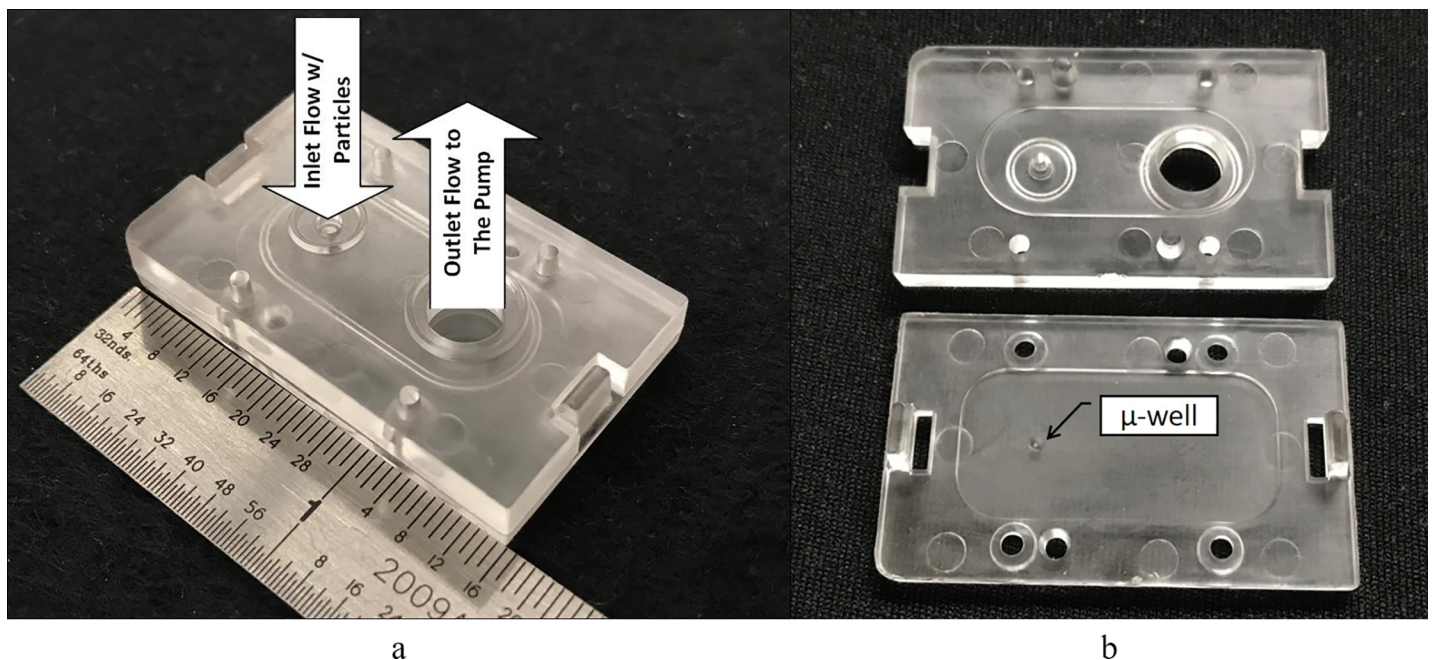
Fig 1. (a) The photograph of the assembled \mu -well aerosol collection cartridge and (b) the cartridge in a disassembled state.
