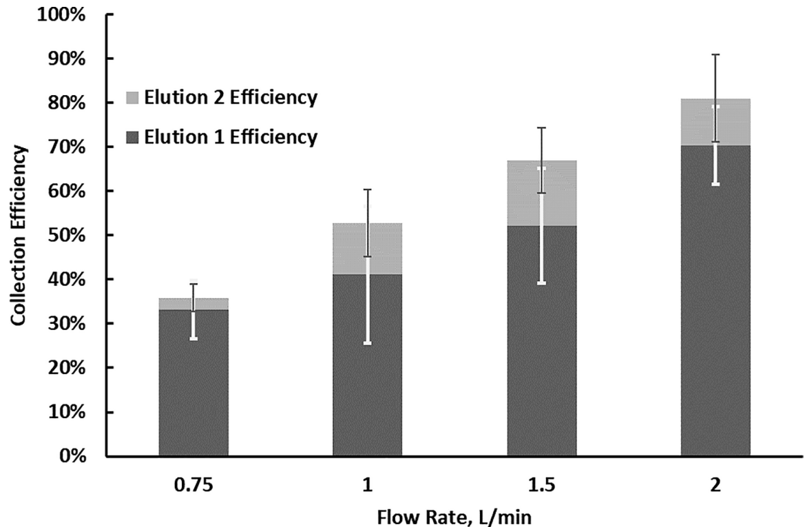
Fig 5. B. subtilis collection efficiencies in \mu -well inertial impactors as a function of the collector flow rate.
