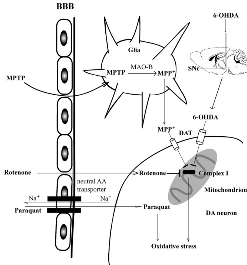
Figure 2. The administration routes and lesion mechanisms of dopaminergic neurotoxins. 6-OHDA must be delivered via intracerebral injection into SNc or striatum, where it is transported into dopaminergic neurons by DAT. MPTP, rotenone, and paraquat are systemically administered because they can cross the BBB. MPTP is metabolized by MAO-B in glial cells to MPP + , which is also transported into dopaminergic neurons by DAT. Rotenone directly enters the dopaminergic neurons due to its hydrophobicity. 6-OHDA, MPP + , and rotenone inhibit the activity of complex I and further result in dopaminergic neurodegeneration. Neutral amino acid transporter mediates the Na + -dependent entry of paraquat into dopaminergic neurons, where it impairs the redox recycling and induces oxidative stress, ultimately leads to the neuronal death.
