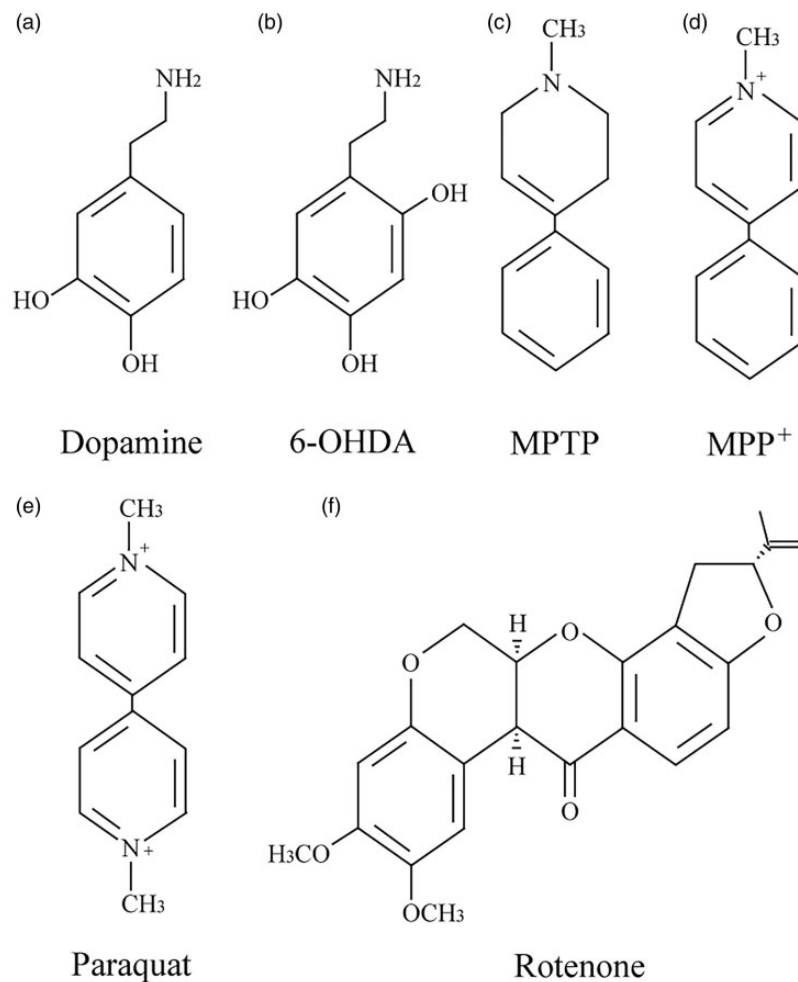
Figure 1. Structures of dopamine and main neurotoxins used to reproduce features of PD in animal models. 6-OHDA = 6-hydroxydopamine; MPTP = 1-methyl-4-phenyl-1,2,3,6-tetrahydropyridine; MPP + = 1-methyl-4-phenylpyridinium ion.
