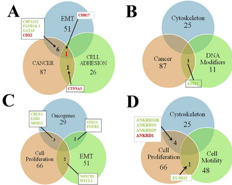
Fig. 4. Slit2 microarray results in Venn diagrams arrangements. We generated Venn diagrams from our microarray as a way of representing group of genes affected by Slit2. A shows diagram for EMT, cancer and cell adhesion molecules. CDH17 was the only common gene among these three groups. B shows cytoskeleton, cancer and DNA modifiers, we only found EZH1 gene from cancer and DNA modifiers combined. C shows oncogenes, EMT and cell cycle gene arrangement. We did not have a triple positive among the three but NOTCH1 and MYCL1 between EMT and cell cycle. D shows cytoskeleton, cell cycle and cell motility combination. Here Ankyrins were common among cell cycle and cytoskeleton, while between cell cycle and motility only ELMO was the common gene. Names in red indicates upregulated genes, in green, downregulated.
