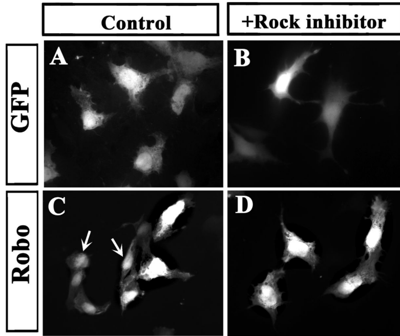
Fig. 7. ROCK inhibition reverses Robo GOF and LOF phenotype. Chicken neural tubes (HH14–15) were electroporated with control-GFP or Robo plasmids, isolated and cultured for 24 h. A, C shows GFP staining of cells under control conditions and B, D cells treated with ROCK inhibitor. Control GFP cells showed classic mesenchymal, more extended shape while many Robo cells did not exhibit mesenchymal shape but a more rounded one (arrows in C ). After ROCK inhibitor, GFP control cell remained looking mesenchymal while Robo GOF cell regained a mesenchymal/migratory shape ( D ).
