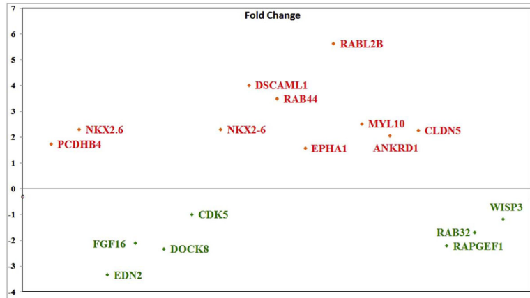
Fig. 3. Genes with marked expression. Genes with substantial expression difference of -2 < x > +2 between control and Slit2 treatment were graphed.
