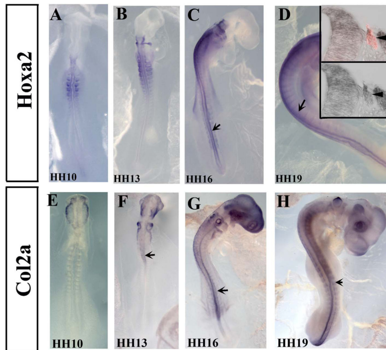
Fig. 5. HoxA2 and Col2a are expressed by pre-migratory and migrating neural crest cells. Wholemount in situ hybridization images of HH10–19 chicken embryos with HoxA2 (A–D) and Collagen2a (E–H) anti-sense probes. Chicken embryos showed expression in neural tubes (arrows in A–H) and migrating neural crest cells (arrowheads in A–H). Sections through mid-trunk showed HoxA2 expression in delaminated, migrating HNK1-positive NCC (insert D' showing in situ and HNK1 in red, and D'' just in situ stain).
