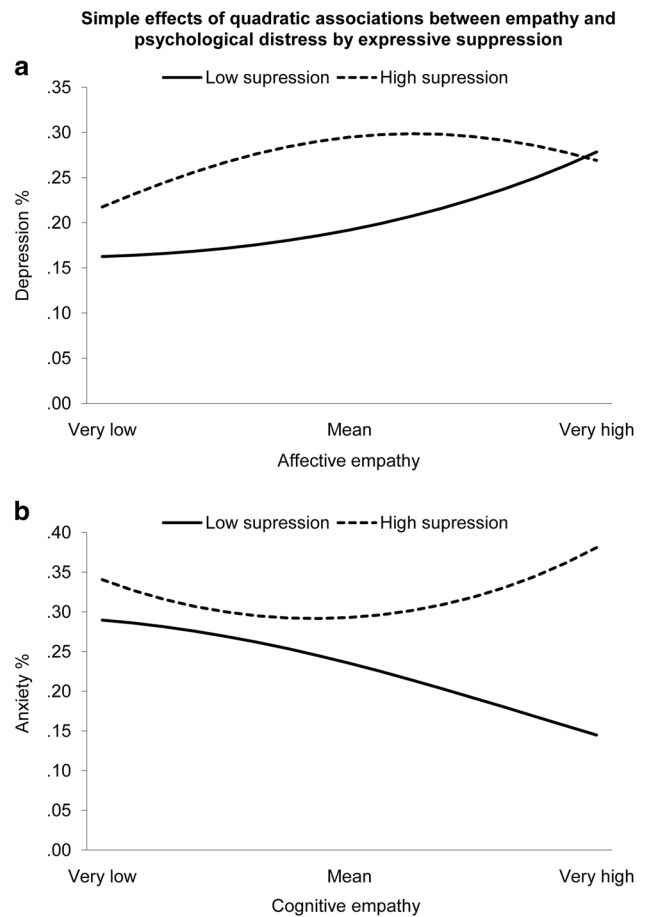
Fig. 2 Simple effects of significant quadratic interactions. Low values of the moderator represent -1 SD , high values represent +1 SD . Slopes graphed between very low ( -2 SD ) and very high ( +2 SD ) levels of the predictor variable
