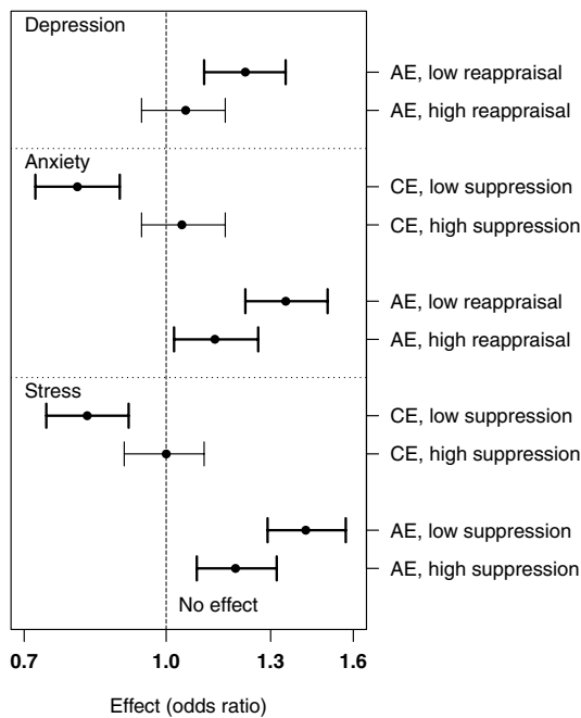
Simple effects of linear associations between empathy and psychological distress by levels of emotion regulation
