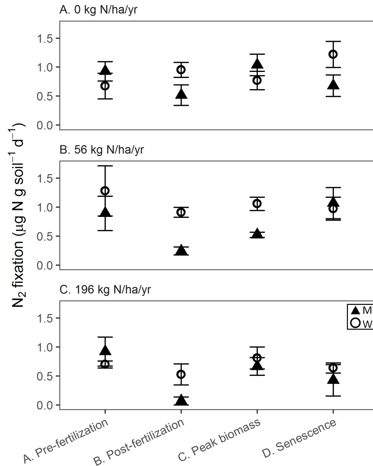
Fig 2. Soil potential ANF rates from two sites (MI: Kellogg Biological Station in Michigan, USA and WI: Arlington Agricultural Research Station, Wisconsin, USA) across four time periods. Soils were sampled from switchgrass rhizospheres grown with a range of N fertilizer addition: A. unfertilized, B. 56 kg N ha -1 yr -1 , and C. 196 kg N ha -1 yr -1 .
