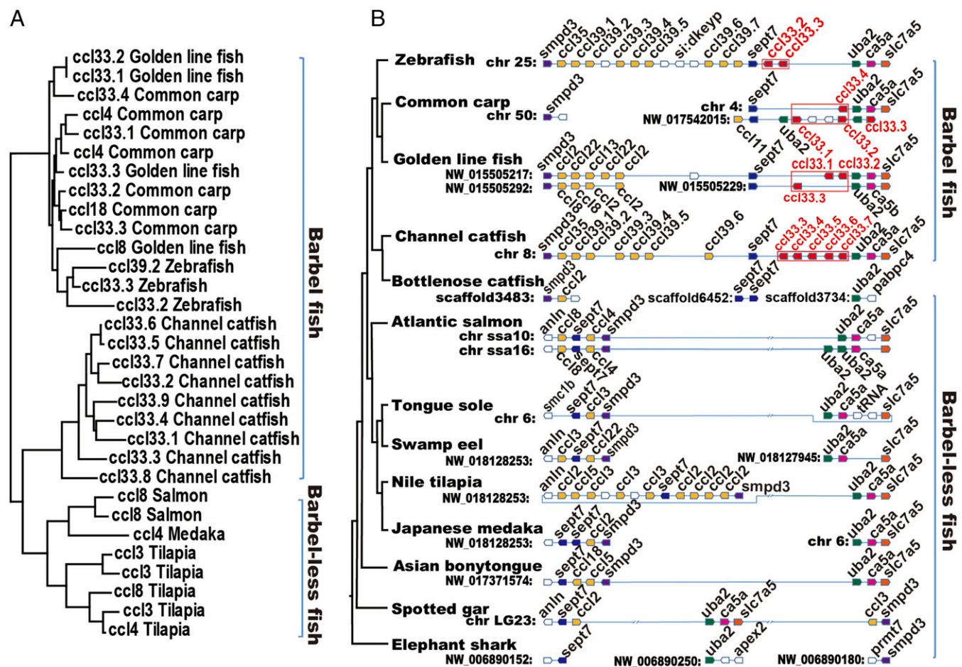
Fig. 2. Chemokine ccl33 genes were identified to be specific in barbeled fish. (A) Phylogenetic clade containing chemokine ccl33 genes was only present in barbeled fish. (B) Conserved syntenic region that included the ccl33 (in red box) genes was specific in barbeled fish.
