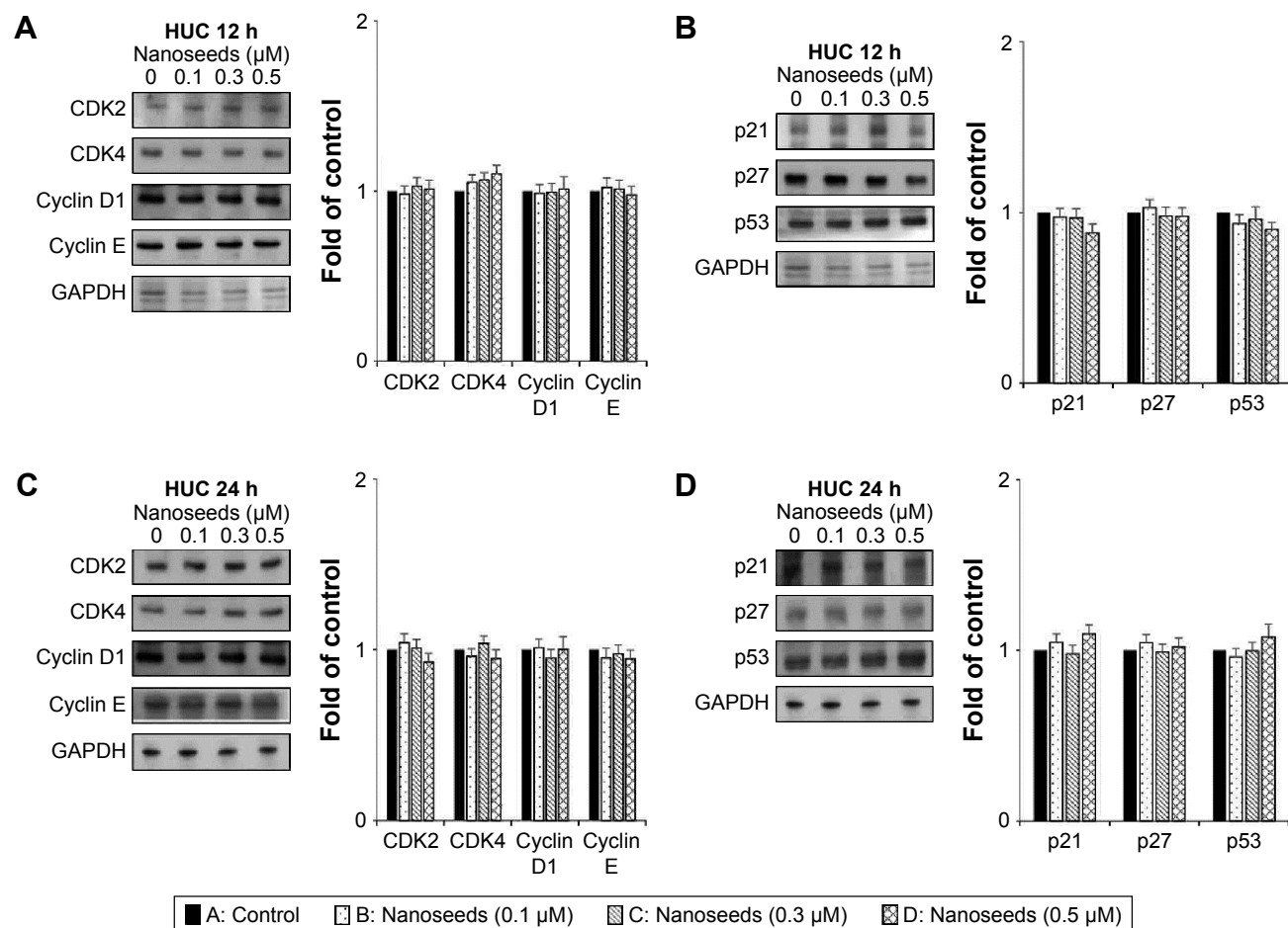
Figure 4 Immunoblots of cell cycle regulators in Au@Pt-NS-treated HUCs.
