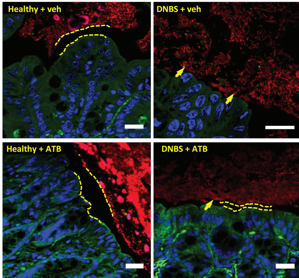
FIGURE 5. ATB-429 restores normal gut microbiota biofilm localization. C57Bl/6 mice were given DNBS intracolonicly to induce colitis, treated orally with ATB-429 (50 mg/kg, twice daily), and killed after 5 days ( n = 8 per group). Intestinal microbiota biofilms were stained by fluorescent in situ hybridization (Eubacteria probe, in red), host nuclei were labeled with To-pro-3 (in blue), and the epithelial host cytoskeleton was stained with an F-actin-FITC antibody (in green). In animals with colitis, bacteria invaded the mucus layer and adhered to epithelium (arrows), whereas in healthy and in ATB-429-treated mice, the microbiota remained separated from the epithelial surface by a normal mucus layer. Dashed lines represent the sterile mucus layer. Scale bars represent 20 \mu\text{m} .
